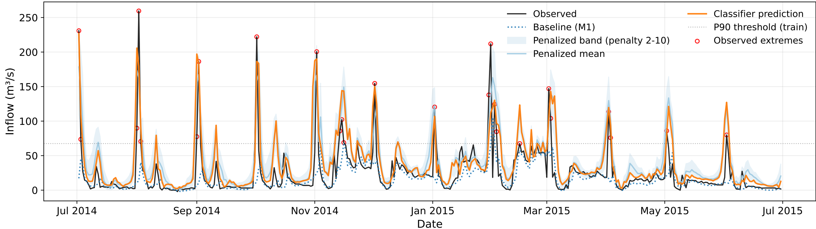
Inflow Forecast 2014 - M5 - Loss: Pinball p=2-10 - Meta-Learner: RF
