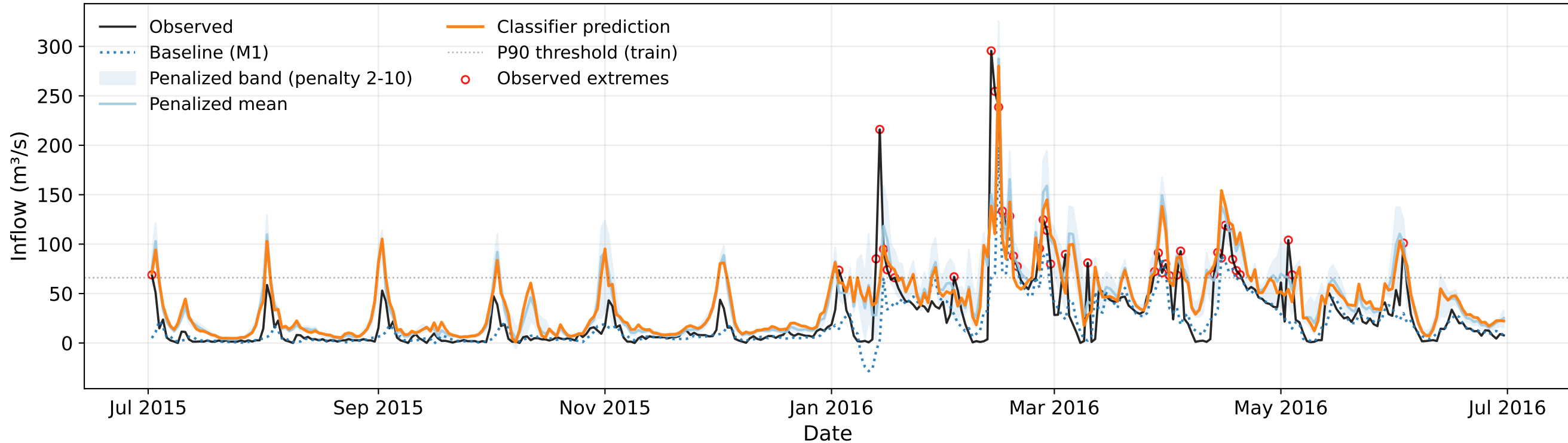
Inflow Forecast 2015 - M5 - Loss: Pinball p=2-10 - Meta-Learner: RF
