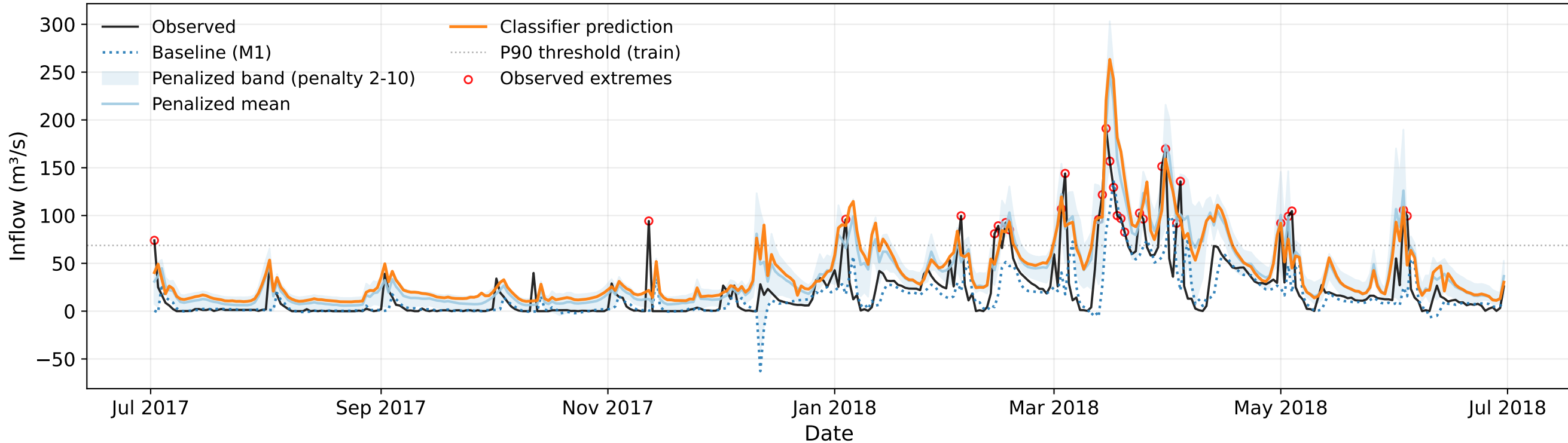
Inflow Forecast 2017 - M5 - Loss: Pinball p=2-10 - Meta-Learner: RF
