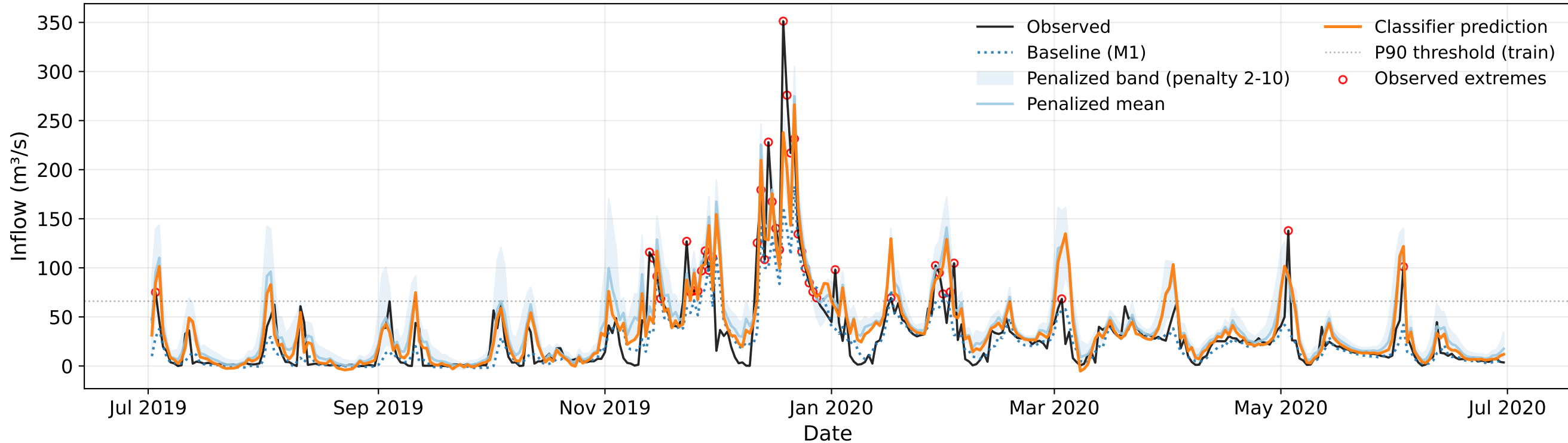
Inflow Forecast 2019 - M5 - Loss: Pinball p=2-10 - Meta-Learner: RF
