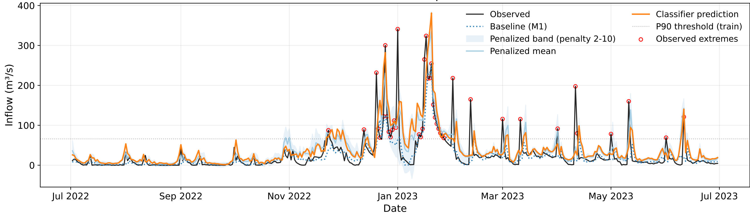
Inflow Forecast 2022 - M5 - Loss: Pinball p=2-10 - Meta-Learner: RF
