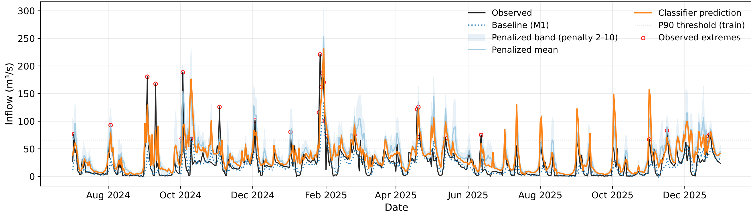
Inflow Forecast 2025 - M5 - Loss: Pinball p=2-10 - Meta-Learner: RF
