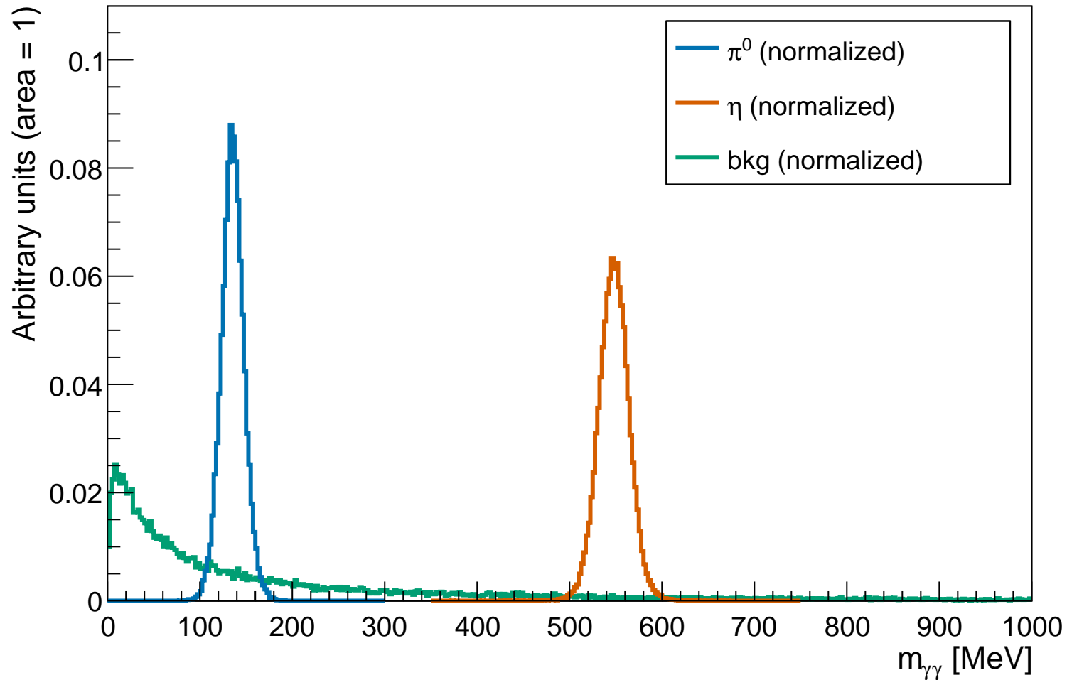
Normalized m_{\gamma\gamma} at L=6.50 cm
