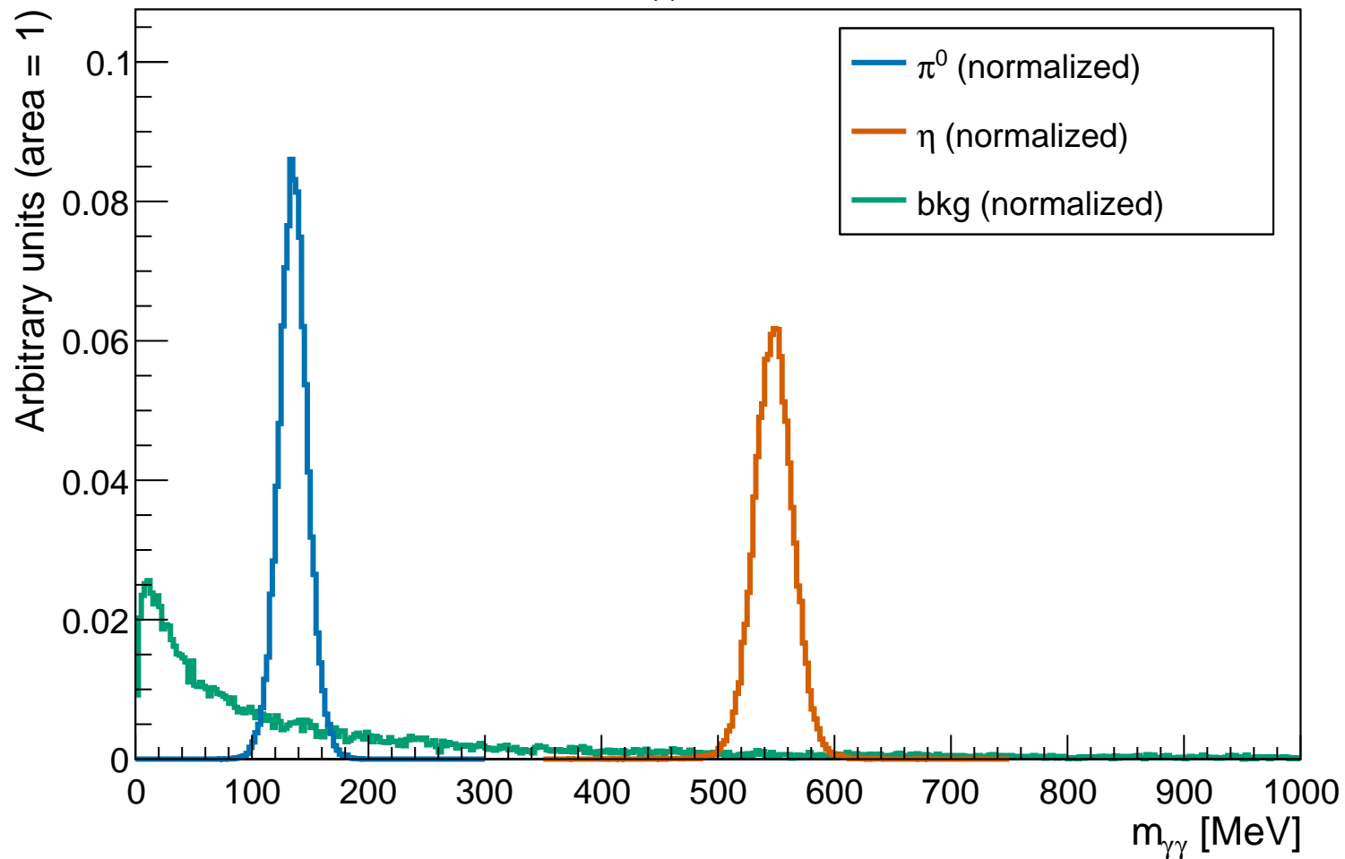
Normalized m_{\gamma\gamma} at L=10.50 cm
