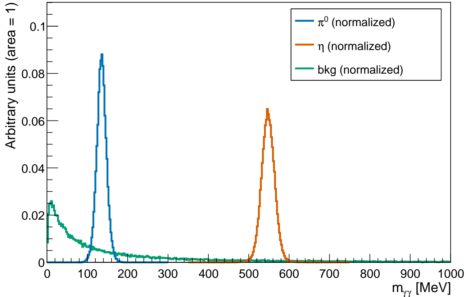
Normalized m_{\gamma\gamma} at L=3.50 cm
