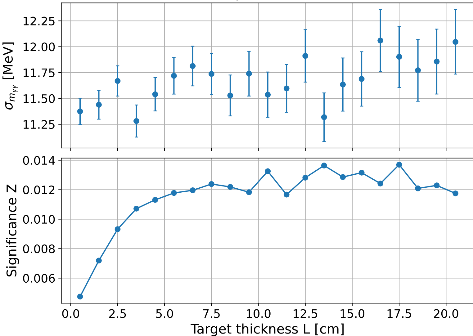
Scan target thickness - \pi^0
