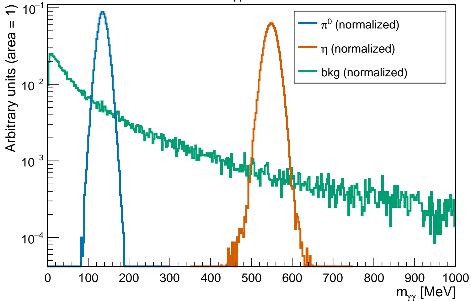
Normalized m_{\gamma\gamma} at L=2.50 cm
