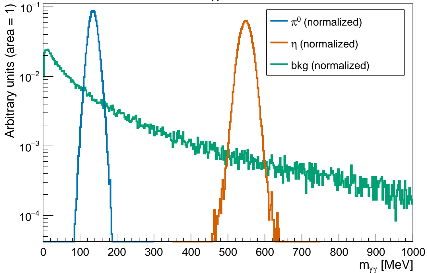
Normalized m_{\gamma\gamma} at L=0.50 cm
