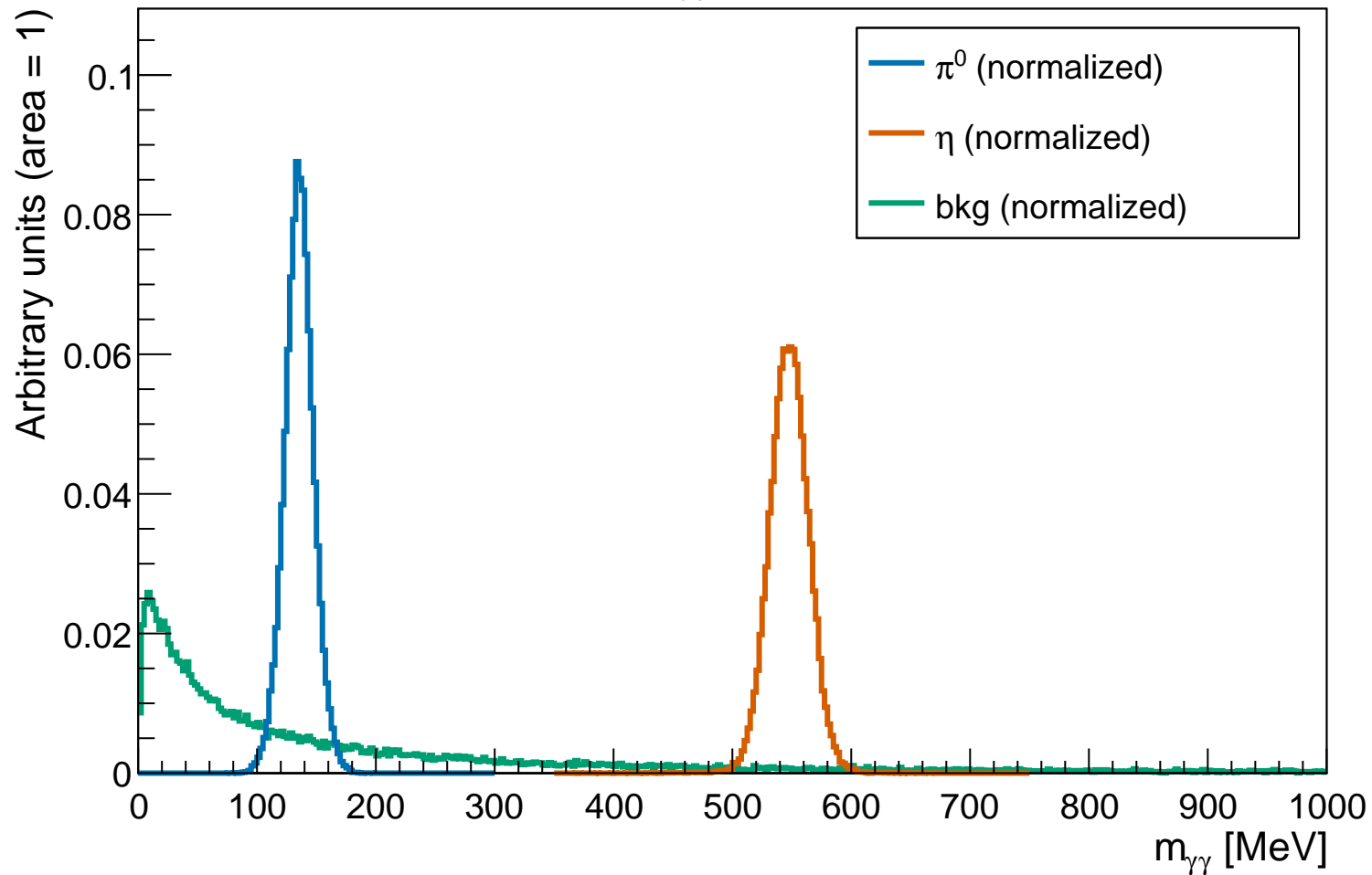
Normalized m_{\gamma\gamma} at L=4.50 cm
