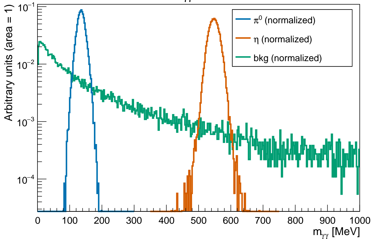
Normalized m_{\gamma\gamma} at L=8.50 cm
