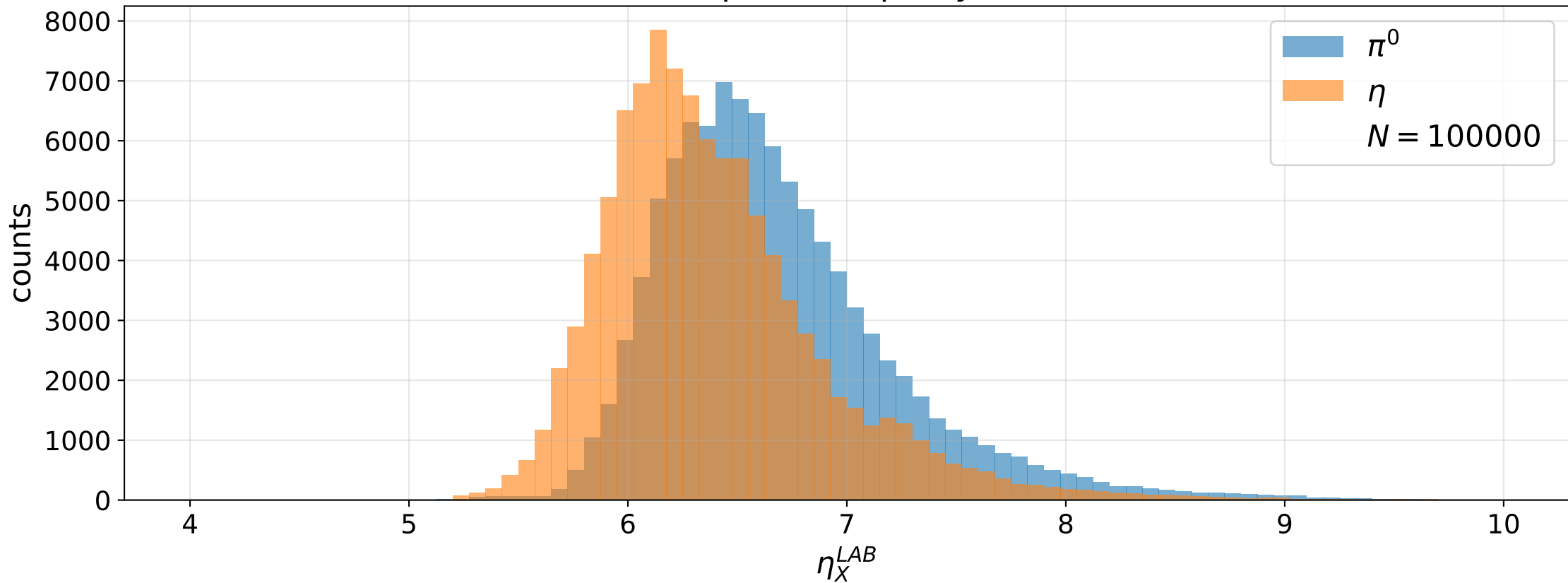
Meson pseudorapidity in LAB
