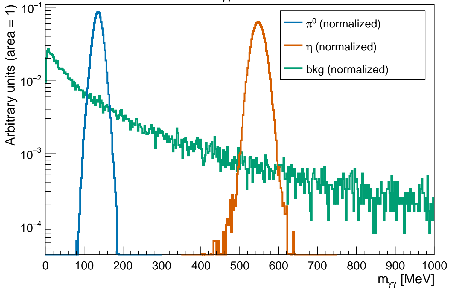
Normalized m_{\gamma\gamma} at L=5.50 cm
