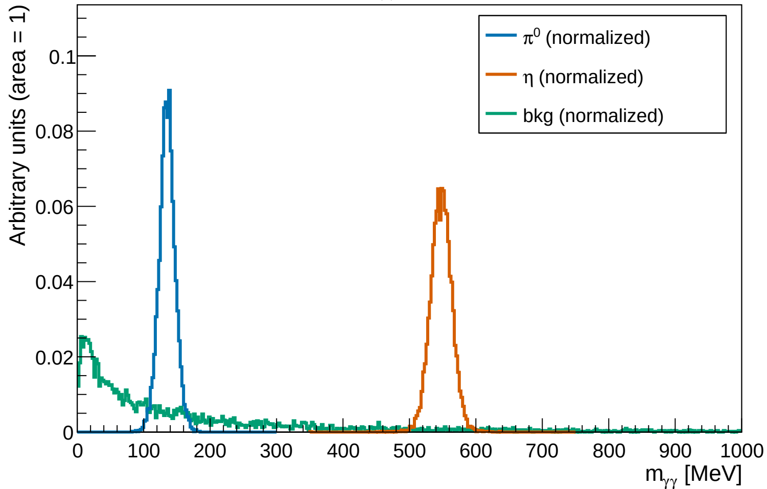
Normalized m_{\gamma\gamma} at L=2.00 cm
