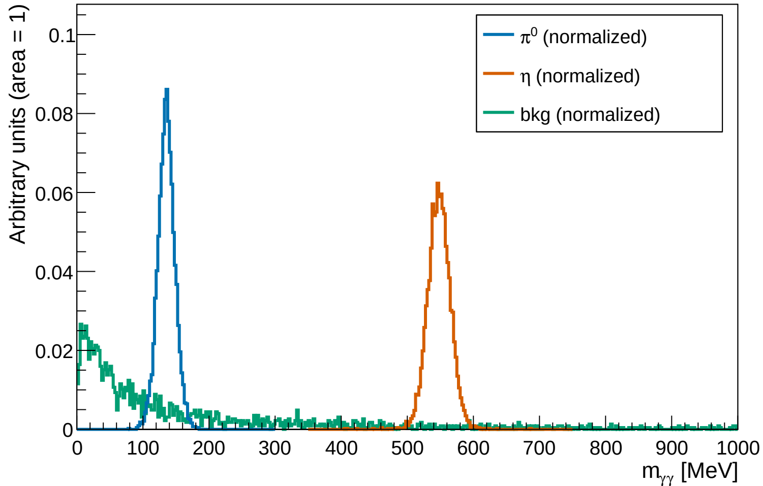
Normalized m_{\gamma\gamma} at L=62.00 cm
