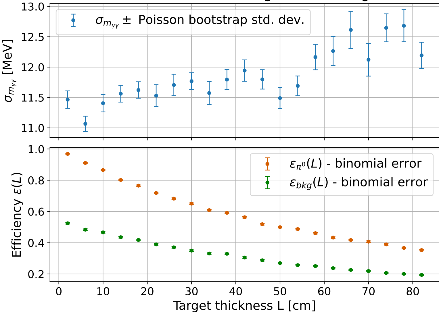
\pi^0 mass resolution; \varepsilon for signal and background
