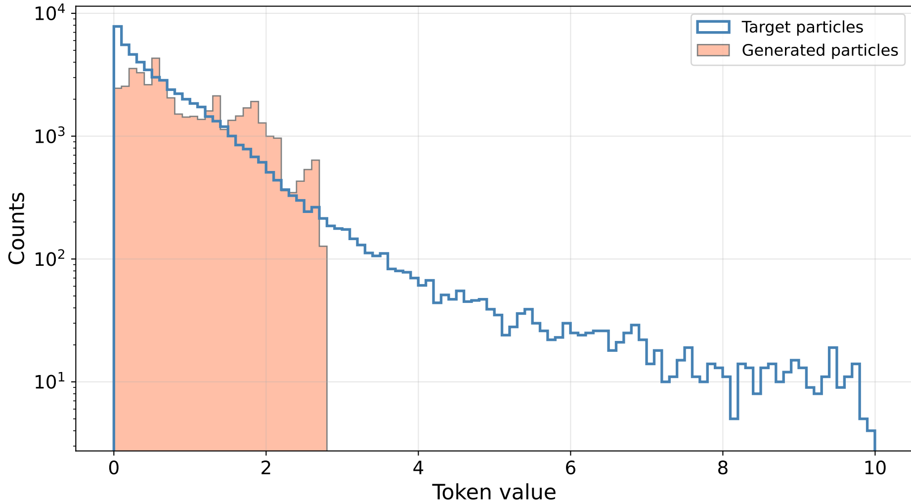
Distribution of tokens values for all the events
