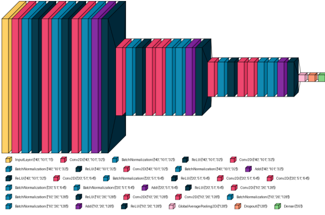
Fig. 2: Block diagram of the Residual CNN architecture.
