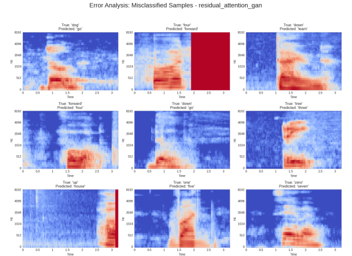
Fig. 8: Examples of misclassified samples by the Residual Attention GAN model.
