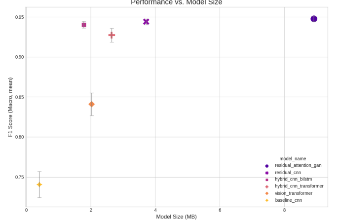
Fig. 4: Trade-off between F1-score and model size.
