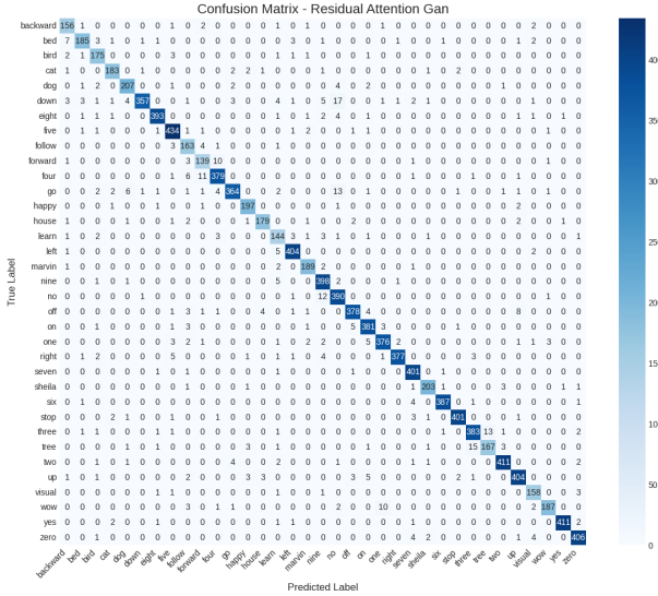
Fig. 6: Confusion matrix for the Residual Attention GAN model
