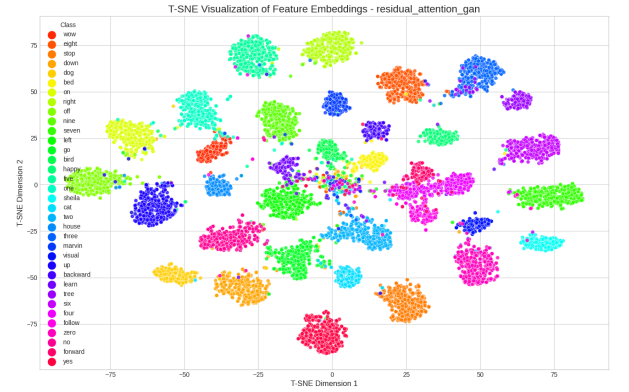
Fig. 7: T-SNE visualization of feature embeddings from the Residual Attention GAN model.
