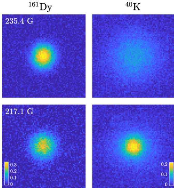
Figure 4.3: Ballistic (upper) and hydrodynamic (lower) expansion of the mixture in the weakly, and strongly interacting regime, respectively. Figure taken from Ref. [28].
