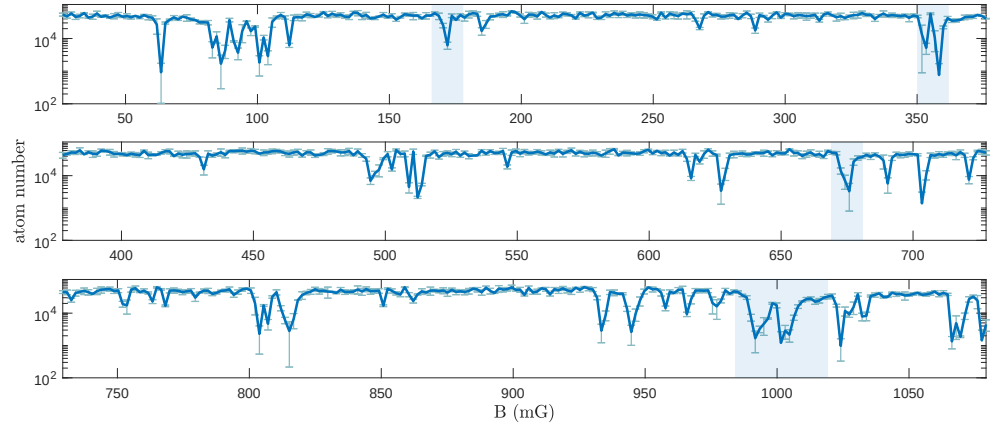
Figure 4.4: Loss spectroscopy of ^{161}\text{Dy} in the lowest hyperfine state. Figure taken from Ref. [33].
