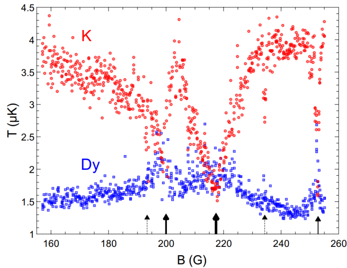
Figure 4.2: Interspecies thermalization scan around the 200 G region. Solid arrows point to the main resonance features. Figure taken from Ref. [32].
