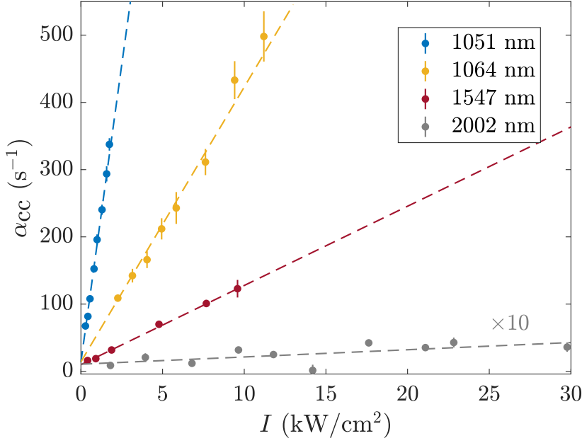
Figure 10.3: Loss rate as a function of the trapping beam peak intensity. We show the closed-channel one-body loss rates measured in the experiments for the 1051.03 nm, 1547.12 nm, and 2002.00 nm ODTs in blue, red and gray dots, respectively. Note that the data and fit result for the 2002-nm case have been scaled by a factor of 10 for better visibility. For comparison, we also show the data for a trap at 1064.04 nm in yellow, already reported in [115]. The data are shown with 1\sigma error bars derived from the lifetime fits (in some cases smaller than the symbol size). For conversion of intensity (in kW/cm 2 ) to optical potential depth (in \mu K) use the factors 1.76, 1.81, 1.25, and 1.15 for the wavelength 1051 nm, 1064 nm, 1547 nm, and 2002 nm, respectively.
