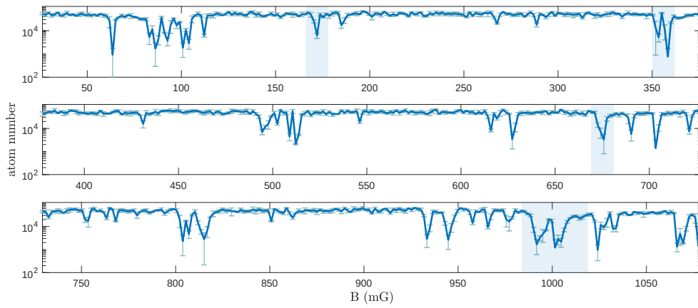
Figure 4.4: Loss spectroscopy of ^{161}\text{Dy} , prepared in the lowest hyperfine state. The ultracold atomic sample, being fermionic and spin polarized, is immune from two-body losses and contact interactions. Minima of atom number are caused by higher partial-waves Feshbach (mostly p-wave) resonances. Figure taken from Ref. [35].
