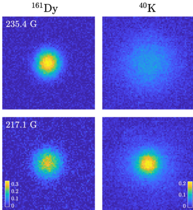
Figure 4.3: Ballistic (upper) and hydrodynamic (lower) expansion of the mixture in the weakly, and strongly interacting regime, respectively. Figure taken from Ref. [9].
