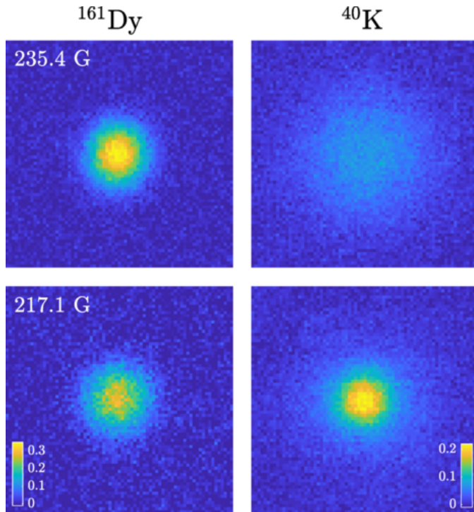
Figure 4.3: Ballistic (upper) and hydrodynamic (lower) expansion of the mixture in the weakly, and strongly interacting regime, respectively. Figure taken from Ref. [29].
