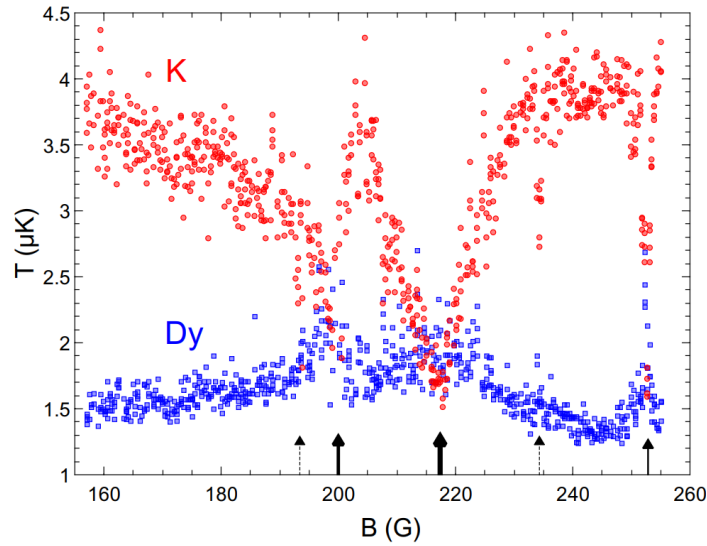
Figure 4.2: Interspecies thermalization scan around the 200 G region. Solid arrows point to the main resonance features. Figure taken from Ref. [6].
