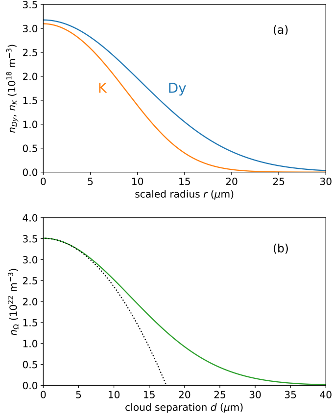
Figure 6.11: Species overlap in the mixture. (a) Spatial profiles for typical experimental conditions N_{Dy} = 5 \times 10^4 , N_K = 2 \times 10^4 , T = 100 \text{ nK} in a spherically symmetric trap with mean frequencies \bar{\omega}_{Dy}/2\pi = 37 \text{ Hz} and \bar{\omega}_K/2\pi = 112 \text{ Hz} . The reduced temperatures T_{Dy}/T_F^{Dy} = 0.84 and T_K/T_F^K = 0.38 correspond to moderate Fermi degeneracy. (b) Overlap integral n_\Omega as a function of a spatial displacement between the cloud centers (solid line) with a second-order Taylor expansion (dotted line).
