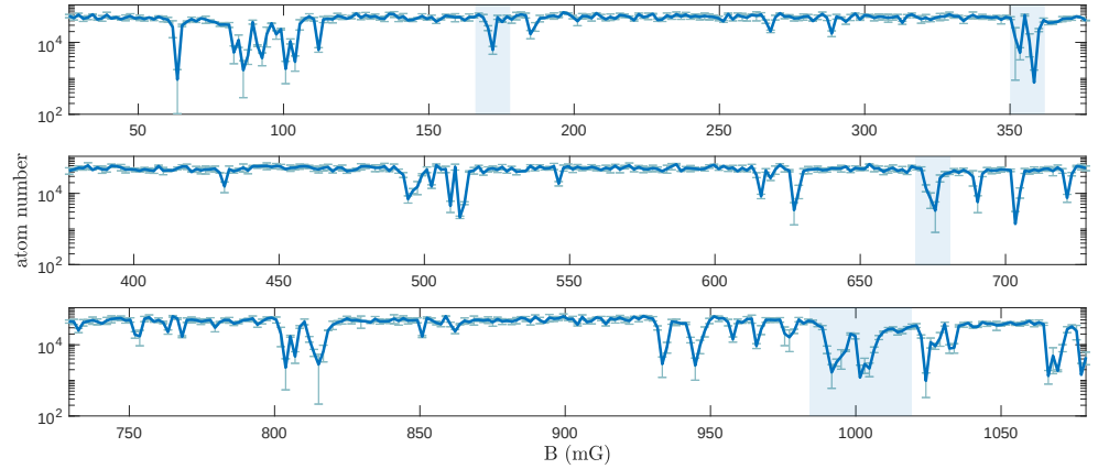
Figure 4.4: Loss spectroscopy of ^{161}\text{Dy} in the lowest hyperfine state. Figure taken from Ref. [7].
