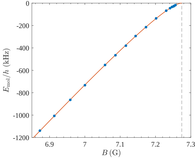
Figure 9.4: Molecular state energy as a function of the magnetic field, measured via modulation of the magnetic field (wobble spectroscopy). The experimental data have been corrected by the small thermal shift of \sim 5 kHz. Uncertainties are smaller than the symbol size. The solid line is a fit to the data according to Eq. (10.2). The dashed line indicates the position of the resonance pole.
