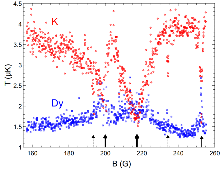
Figure 4.2: Interspecies thermalization scan around the 200 G region. Solid arrows point to the main resonance features. Figure taken from Ref. [5].
