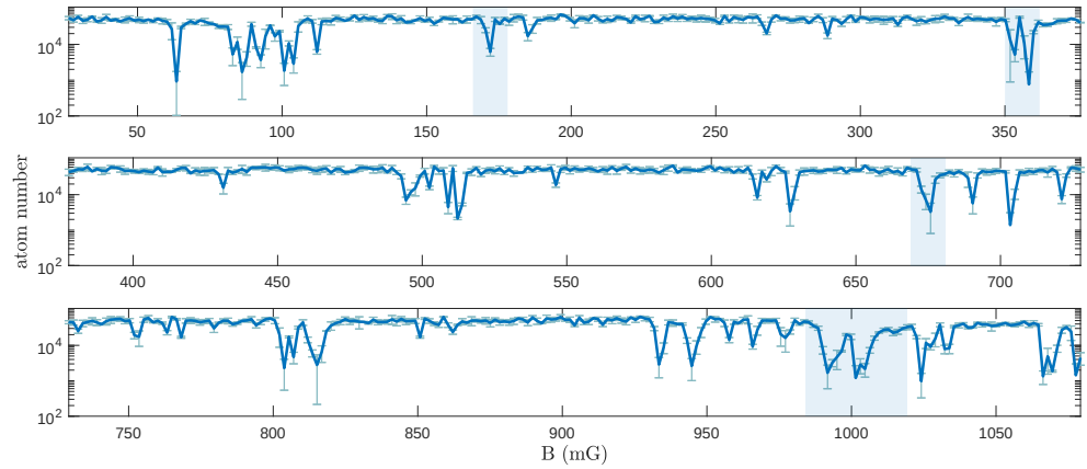
Figure 4.4: Loss spectroscopy of ^{161}\text{Dy} in the lowest hyperfine state. Figure taken from Ref. [6].
