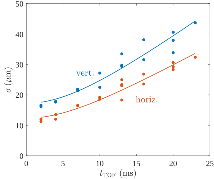
Figure 9.3: Vertical and horizontal size of the molecular cloud as a function of the time of flight t_{\text{TOF}} . The sample is let expand at B = 7.22 G, upon switching off the magnetic levitation together with the ODT. A fit to the data, assuming a ballistic expansion, yields a vertical and horizontal temperature of 77(6) and 45(3) nK, respectively.
