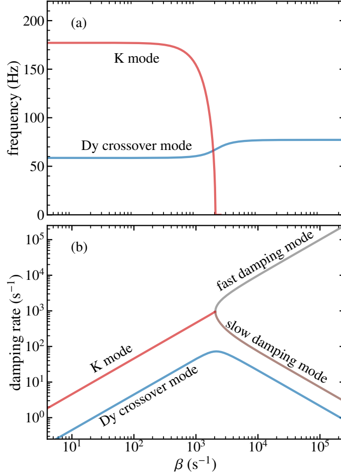
Figure 6.1: Predictions of the theoretical model for the dependence of dipole-mode frequencies (a) and damping rates (b) on the friction parameter \beta . Here we assume \kappa = 0 (no reactive coupling) and typical experimental conditions ( \omega_{\text{Dy}}/2\pi = 59 Hz, \omega_{\text{K}}/2\pi = 177 Hz, N_{\text{Dy}}/N_{\text{K}} = 2.5 ).
