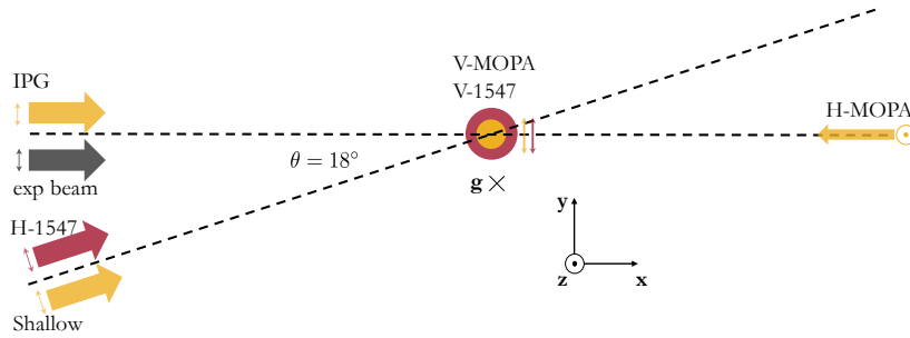
Figure 4.1: ODT setup in the Dy-K experiment. In yellow are reported the trapping beam with a wavelength of 1064 nm, while in red the one with a wavelength of 1547 nm. The gray path is for all the other different ODTs tested during the years and reported in Chapter 10 . Double arrows and the circle-dot indicate the polarization of the beams, linear and circular respectively.
