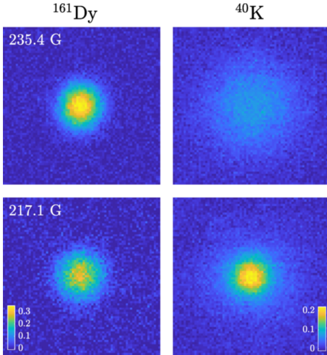
Figure 4.3: Ballistic (upper) and hydrodynamic (lower) expansion of the mixture in the weakly, and strongly interacting regime, respectively. Figure taken from Ref. [23].
