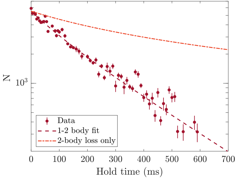
Figure 10.5: Collisional decay and the role of light-induced decay, observed in a 1547-nm trap. The red dots show the number of molecules measured after a variable hold time. The red dashed line represents a fit according to Eq. (10.4). The orange dot-dashed line shows a hypothetical loss curve with the same two-body loss in the complete absence of one-body losses.
