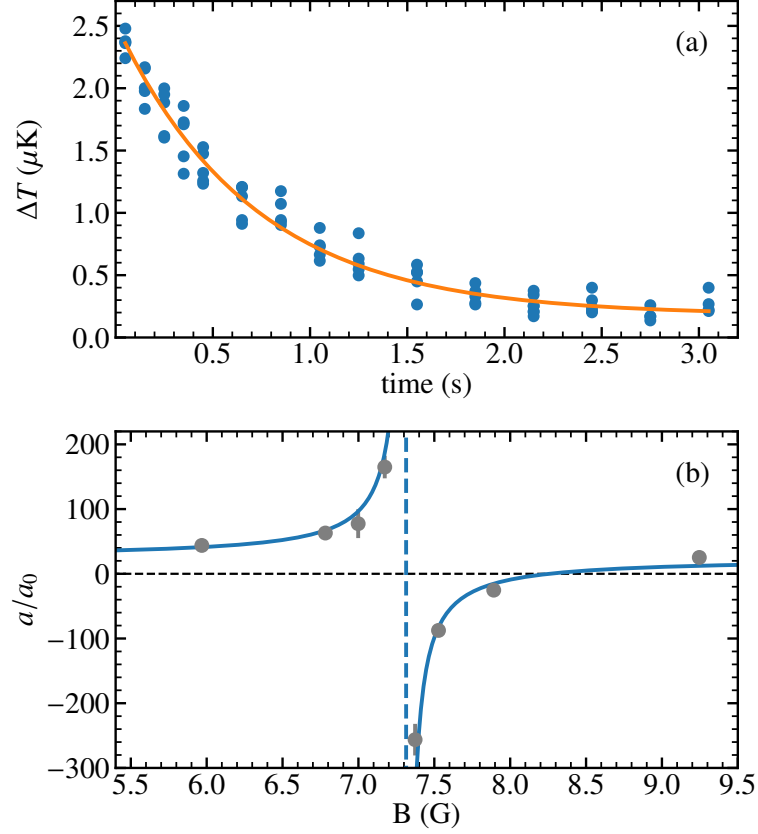
Figure 5.3: Scattering length measurement in the vicinity of the 7.29-G resonance. (a) Temperature difference \Delta T = T_K - T_{\text{Dy}} versus hold time in ODT at 5.97 G. The orange solid line shows the numerical fit curve with the s -wave scattering length a = 53(9)a_0 . (b) Scattering length between Dy and K versus magnetic field strength. The gray points represent the values measured by interspecies thermalization. The solid blue line is a fit based on Eq. (5.1), and the dashed vertical line indicates the pole position.
