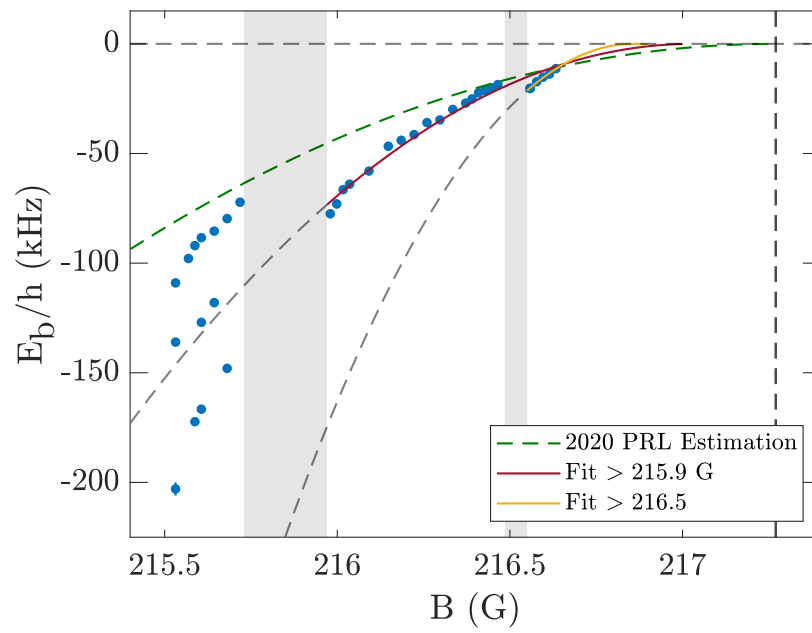
Figure 7.9: Binding energy of Feshbach molecules around the magnetic field region of the 217 G resonance. In red the data point fitted according to eq.5.3
