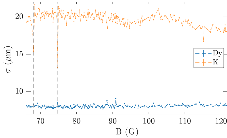
Figure 7.5: Interspecies thermalization scan from 67 G to 120 G.
