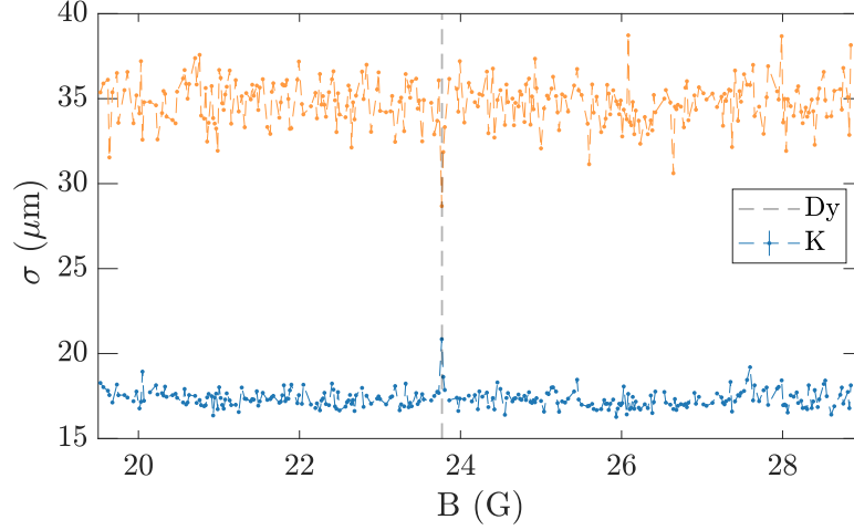
Figure 7.2: Interspecies thermalization scan from 19 G to 29 G. The only resonances identified in this range is indicated by the vertical dashed line.
