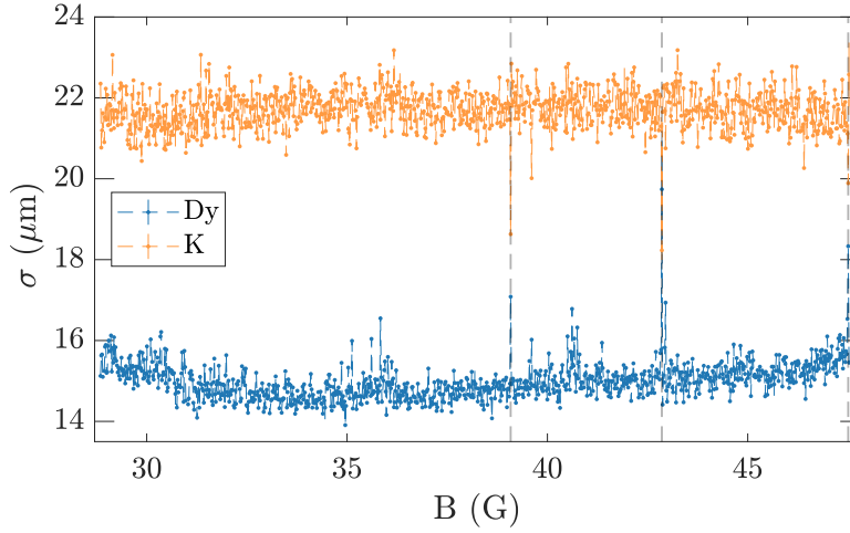
Figure 7.3: Interspecies thermalization scan from 29 G to 47 G. Resonances are indicated by vertical dashed lines.
