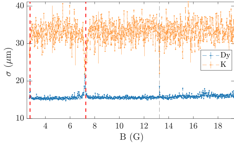
Figure 7.1: Interspecies thermalization scan from 3 G to 19 G. Resonances are indicated by vertical dashed lines, in red the ones already reported in chapter 5. located approximately close to 3 G and 7 G.
