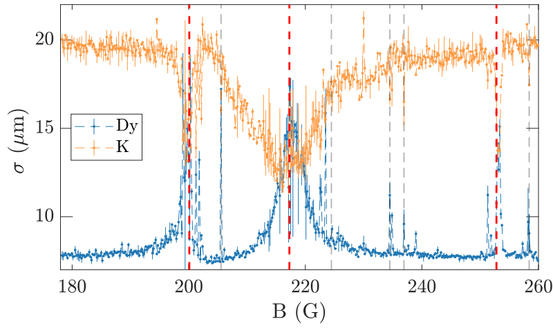
Figure 7.7: Interspecies thermalization scan from 180 G to 260 G. The red dashed lines indicate the resonances reported in ref. [34].
