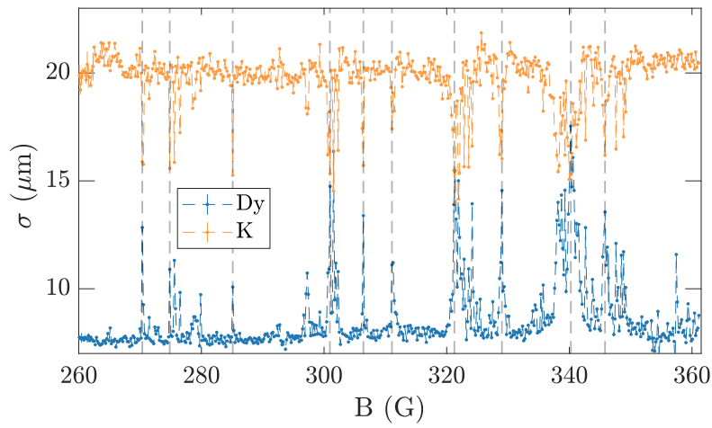
Figure 7.8: Interspecies thermalization scan from 260 G to 360 G.
