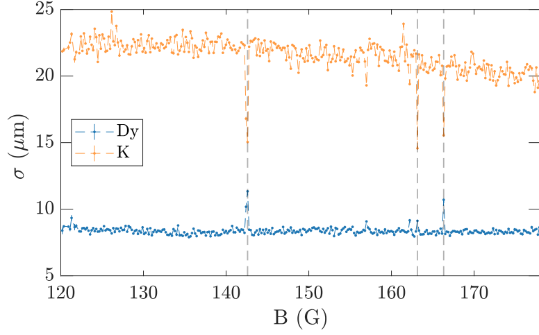
Figure 7.6: Interspecies thermalization scan from 120 G to 180 G.
