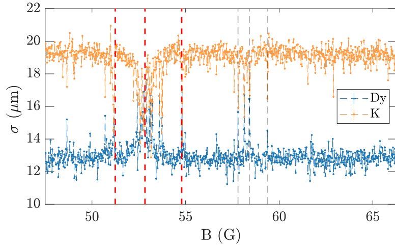
Figure 7.4: Interspecies thermalization scan from 47 G to 67 G. Resonances are indicated by vertical dashed lines. The resonance indicated with the red dashed lines have been already reported. The left most feature at 51.242 G is also reported in chapter 5, while the resonance close to 53 G were already reported in Ref. [39].
