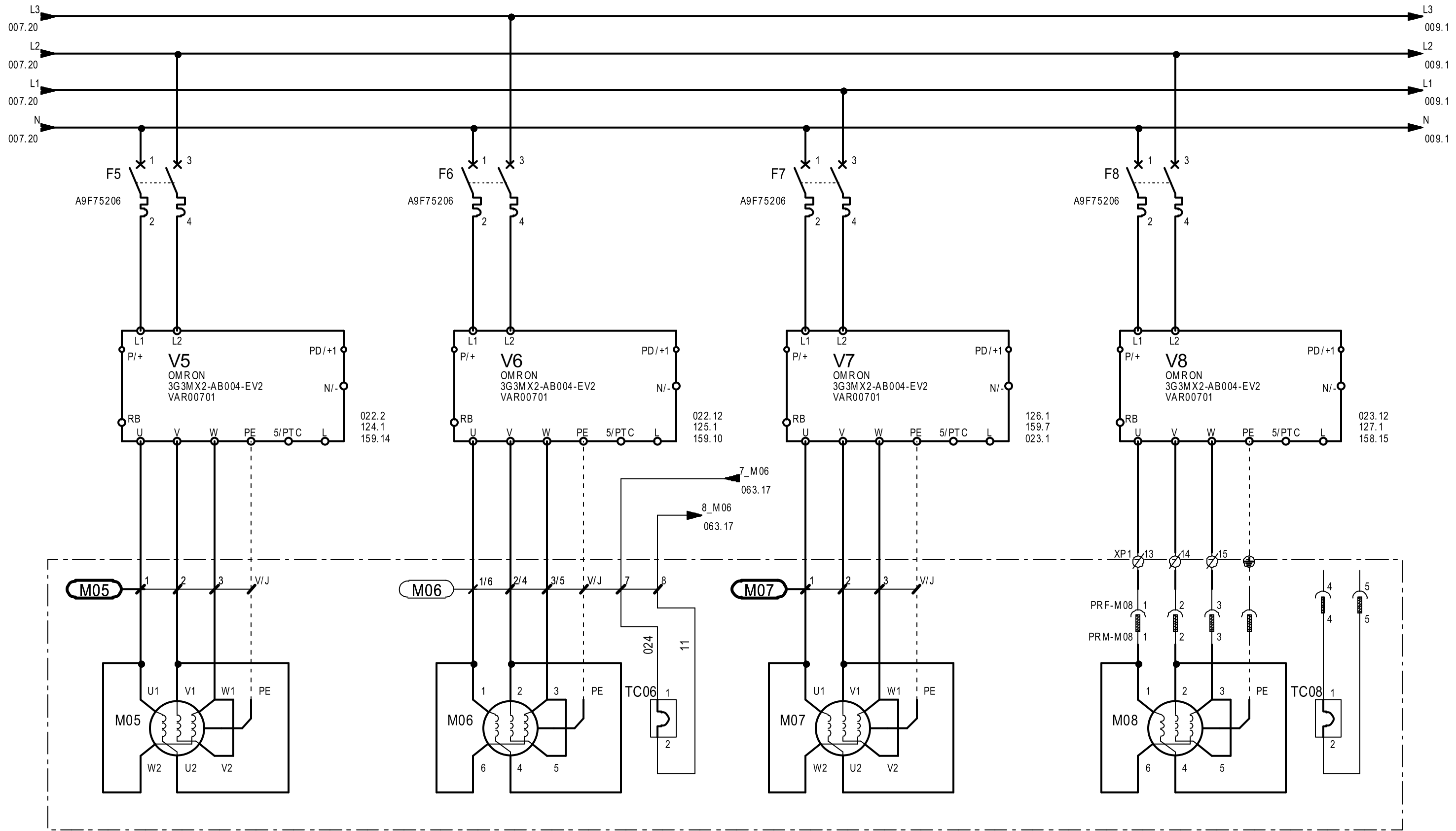
OSCILLATION CONVOYEUR ACCELERATEUR SWINGS ROTATION ACCELERATOR CONVEYOR CONVOYEUR ACQUISITION ACQUISITION CONVEYOR OSCILLATION CONVOYEUR ACQUISITION SWINGS ROTATION ACQUISITION CONVEYOR CONVOYEUR TAPIS ELEVATEUR POUSSIN EN SORTIE CHICK ELEVATEUR OUTFEED 1,26A 1,42A 1,26A 1,30A 0,25KW 230V 50/60 Hz 0,37KW 230V 50/60 Hz 0,25KW 230V 50/60 Hz 0,30KW 230V 50/60 Hz
