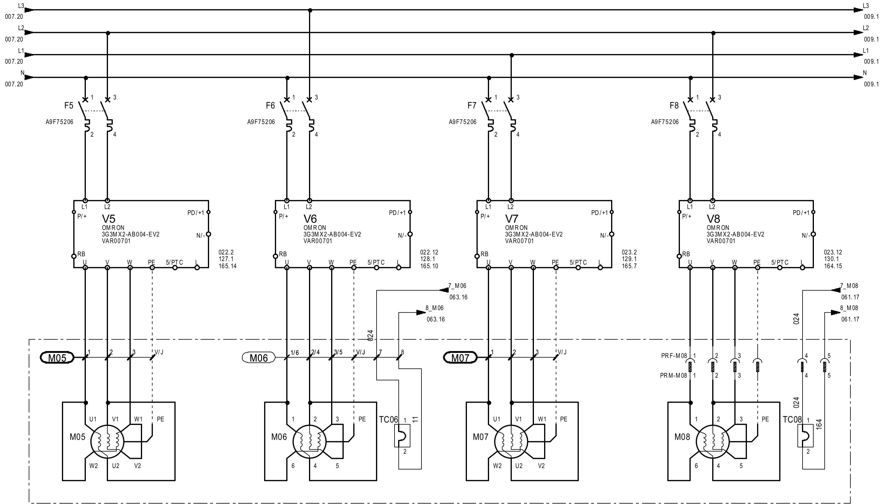
OSCILLATION CONVOYEUR ACCELERATEUR SWINGS ROTATION ACCELERATOR CONVEYOR 1,26A 0,25KW 230V 50/60 Hz
