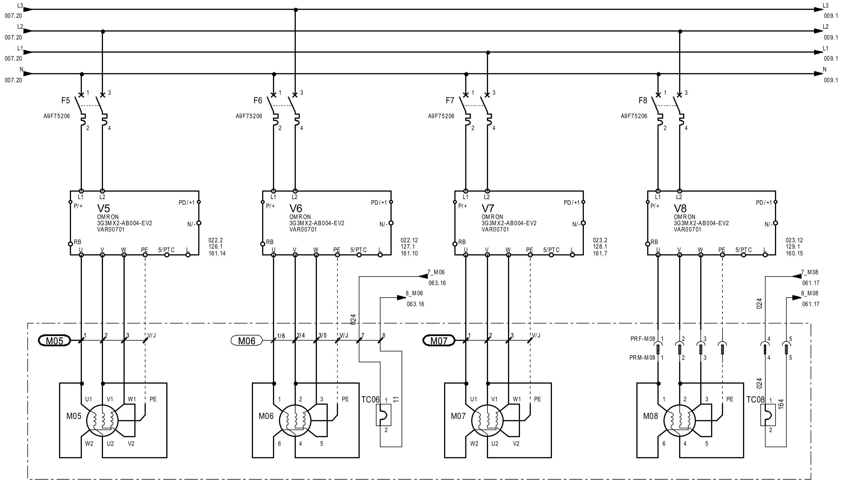
OSCILLATION CONVOYEUR ACCELERATEUR SWINGS ROTATION ACCELERATOR CONVEYOR CONVOYEUR ACQUISITION ACQUISITION CONVEYOR OSCILLATION CONVOYEUR ACQUISITION SWINGS ROTATION ACQUISITION CONVEYOR TAPIS POUSSIN N°1 EN SORTIE CHICK CONVEYOR 1 OUTFEED 1,26A 1,42A 1,26A 1,30A 0,25KW 230V 50/60 Hz 0,37KW 230V 50/60 Hz 0,25KW 230V 50/60 Hz 0,30KW 230V 50/60 Hz
