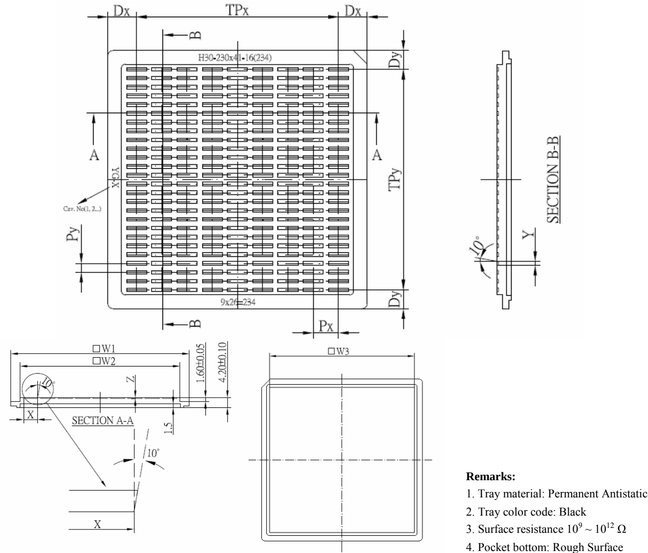
Figure 15-1: SSD1309Z die tray information
