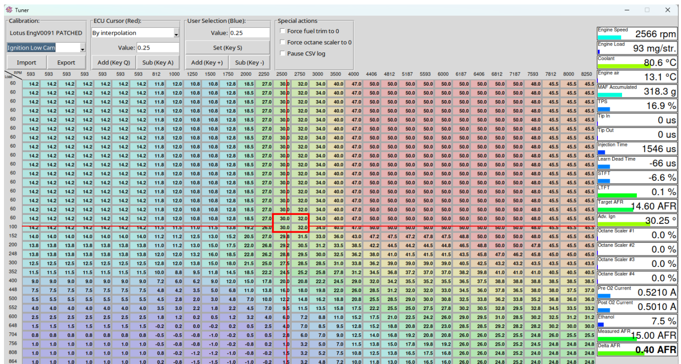
Figure 24: Live ignition map editing over CAN-Bus RAM access on a dyno.
