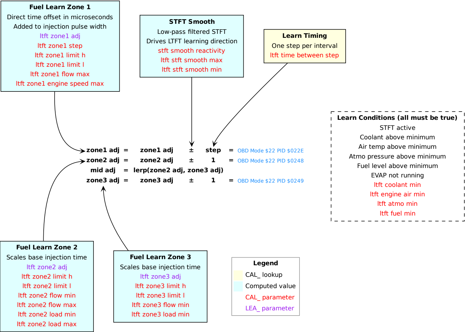
Figure 16: LTFT formula
