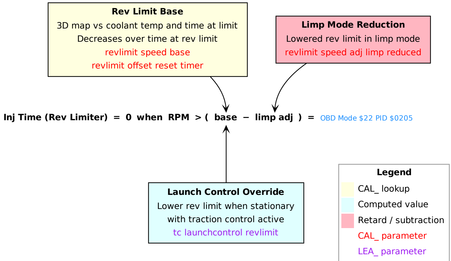
Figure 10: Rev limiter — fuel cut
