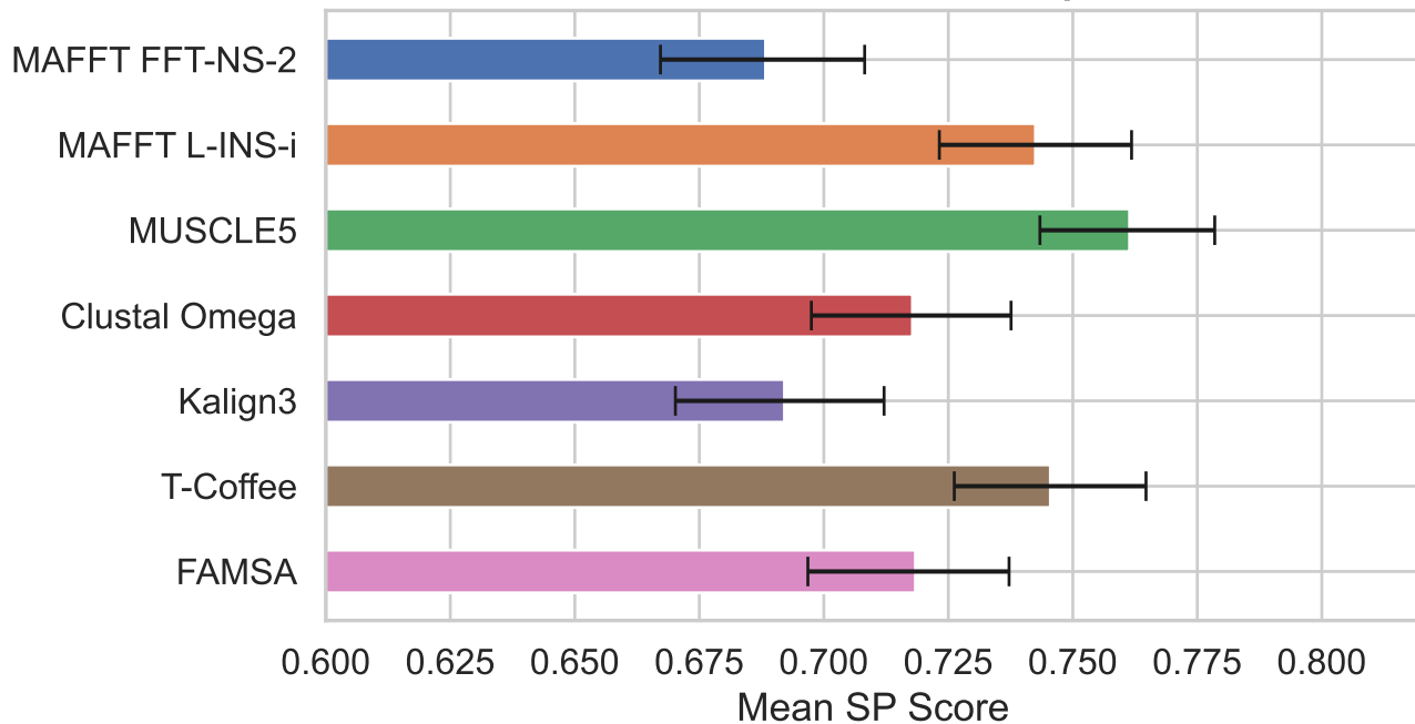
Mean SP Score with Bootstrap 95% CI
