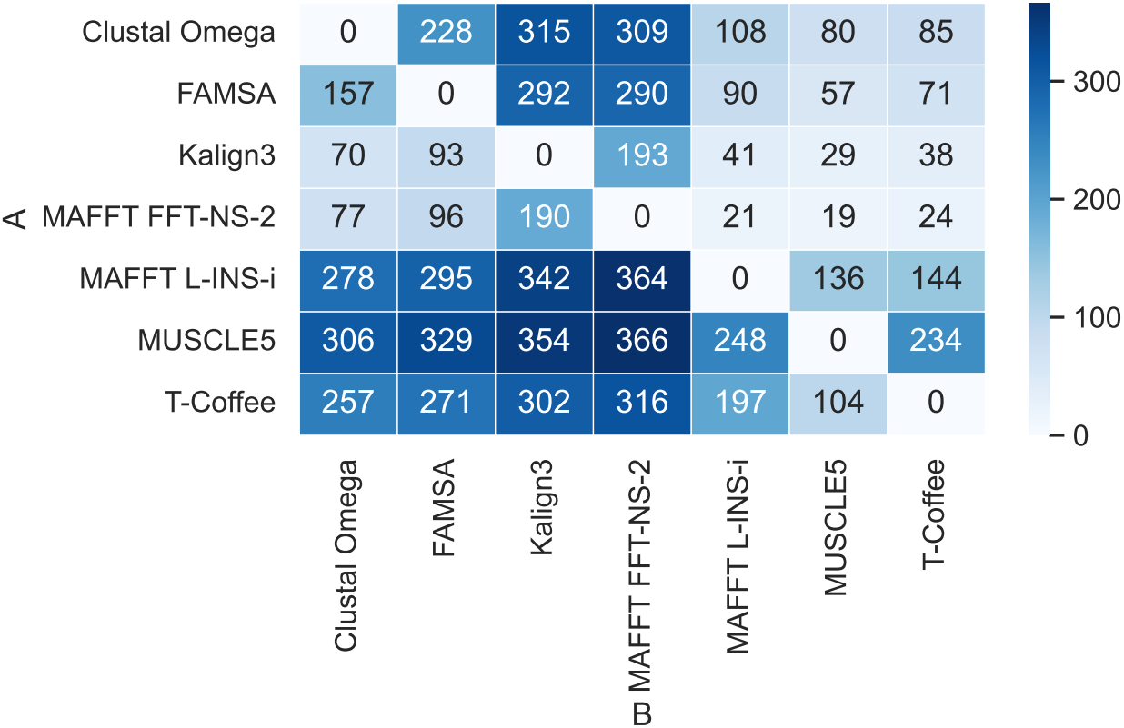
Win Count Matrix (SP Score) row aligner wins over column aligner on N problems
