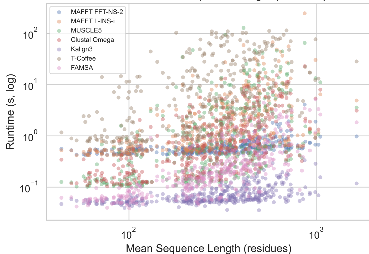
Runtime vs Mean Sequence Length (residues)
