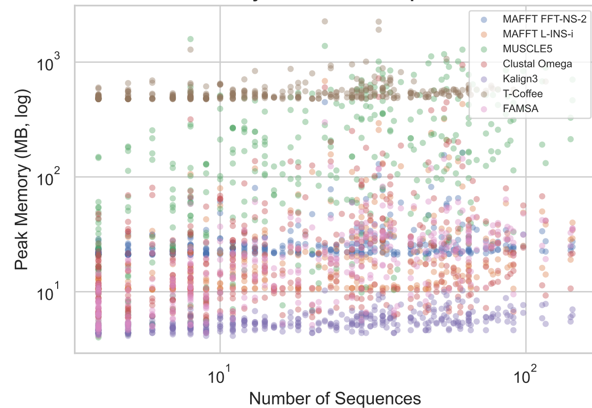
Memory vs Number of Sequences
