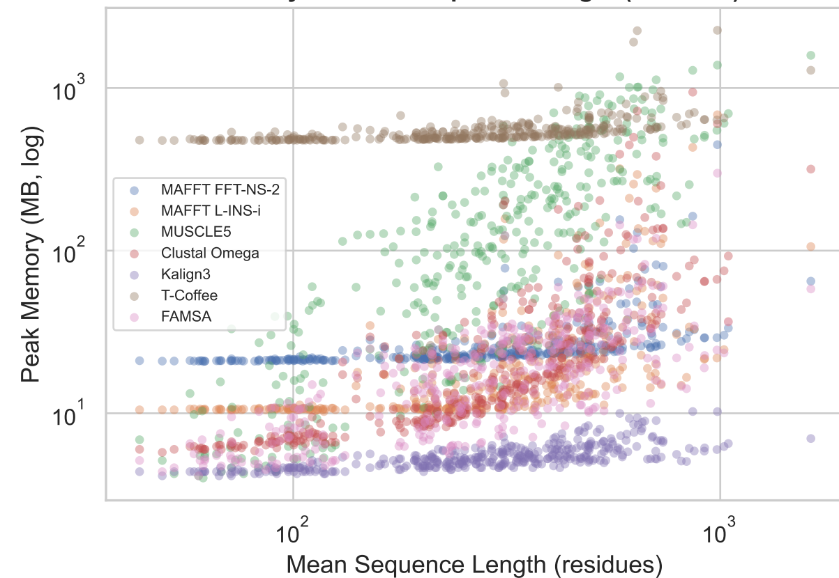
Memory vs Mean Sequence Length (residues)
