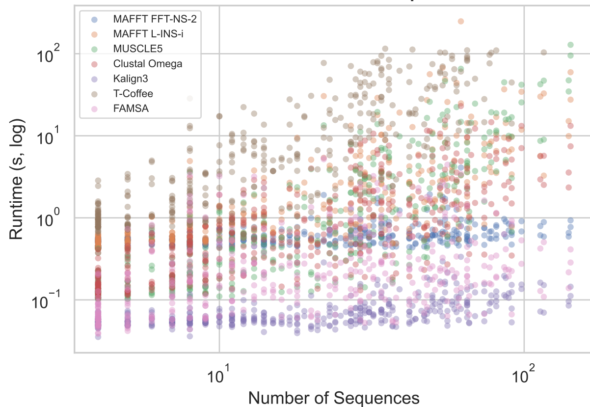
Runtime vs Number of Sequences
