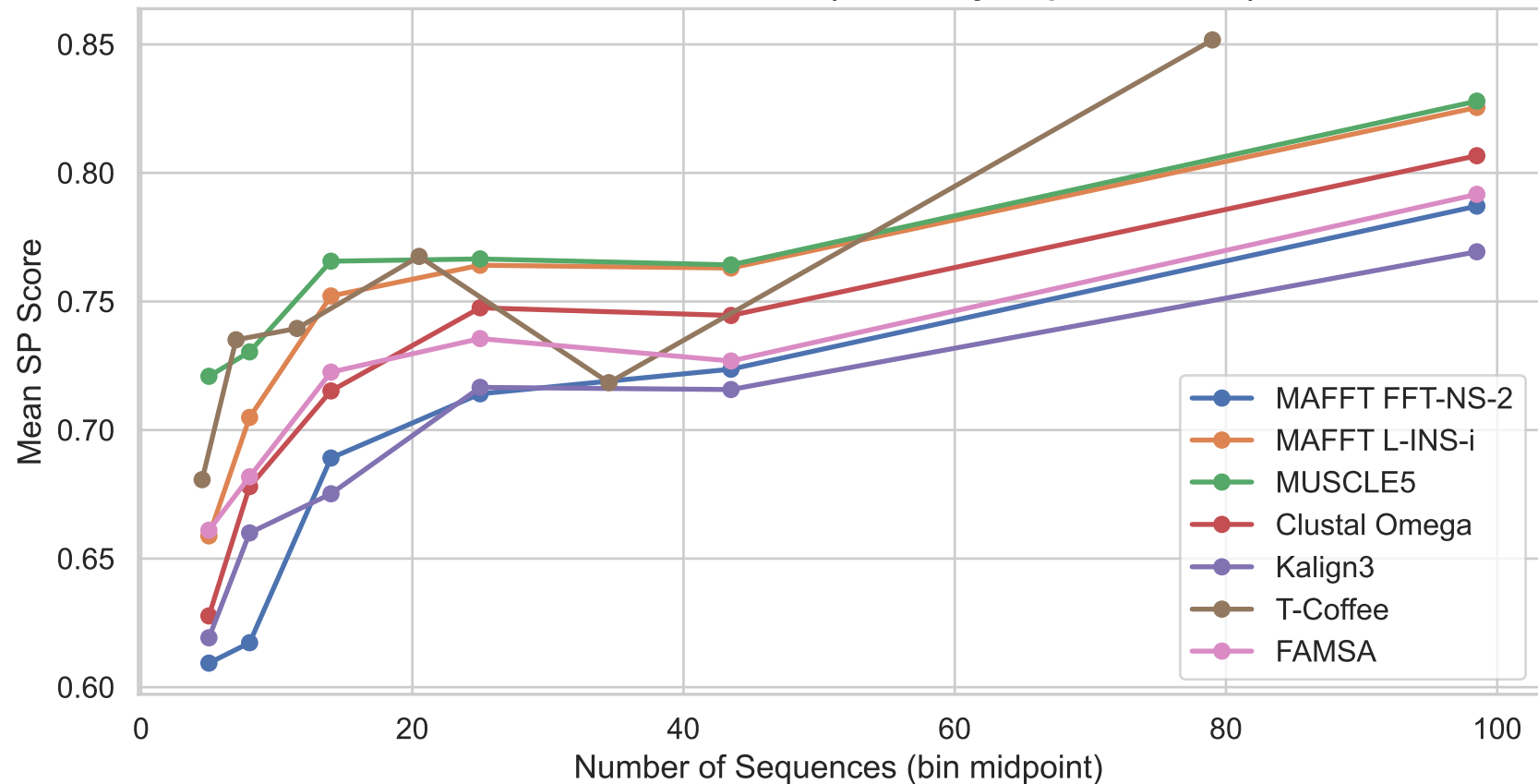
SP Score vs Problem Size (binned by sequence count)
