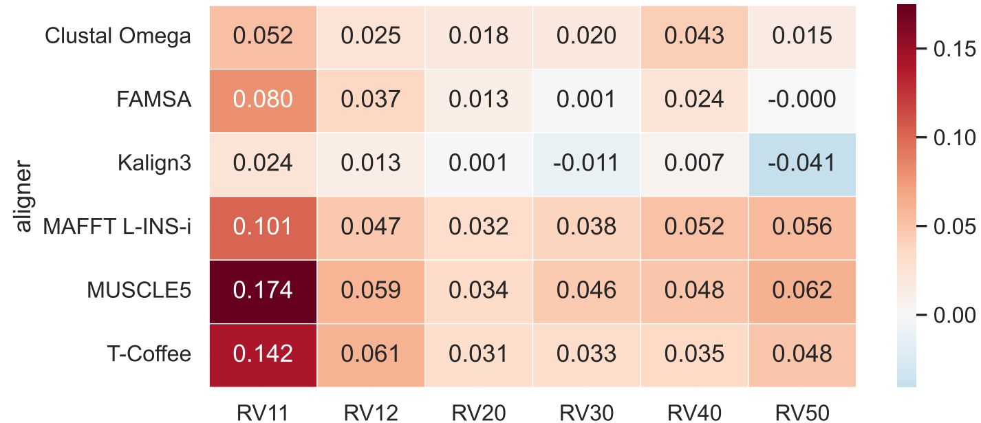
\Delta SP Score vs MAFFT FFT-NS-2 by Reference Set (positive = row aligner scores higher)
