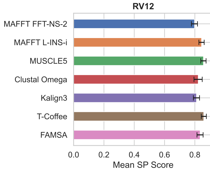
Bootstrap 95% CI on Mean SP Score by Reference Set
