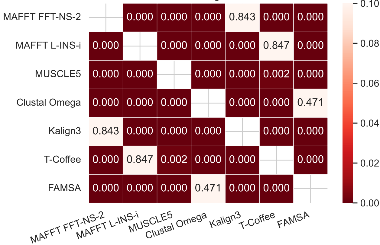
Exact Nemenyi Post-hoc p-values (SP Score) cells below 0.05 indicate significant rank difference
