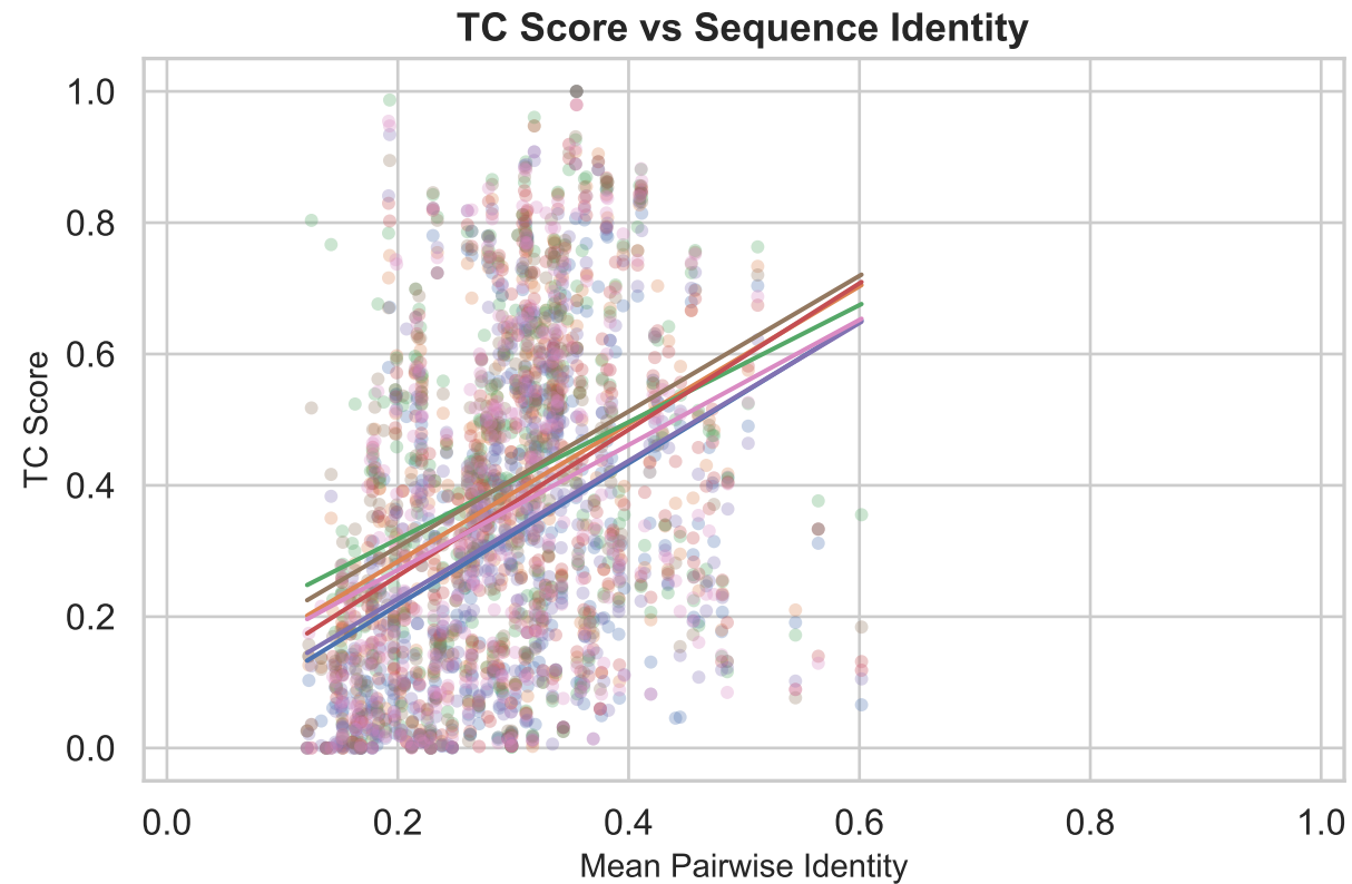
Alignment Accuracy vs Mean Pairwise Sequence Identity (each point = one problem, lines = linear trend per aligner)
