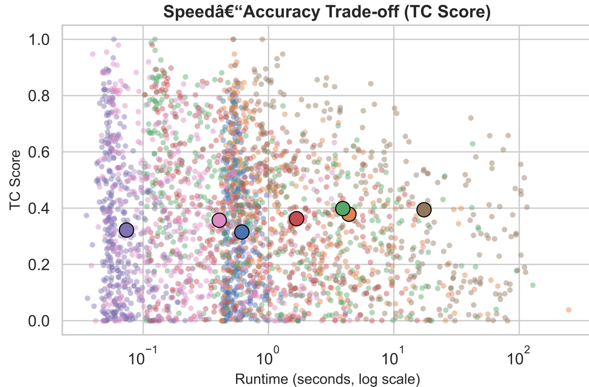
Pareto Plot: Runtime vs Alignment Accuracy (large marker = mean per aligner)
