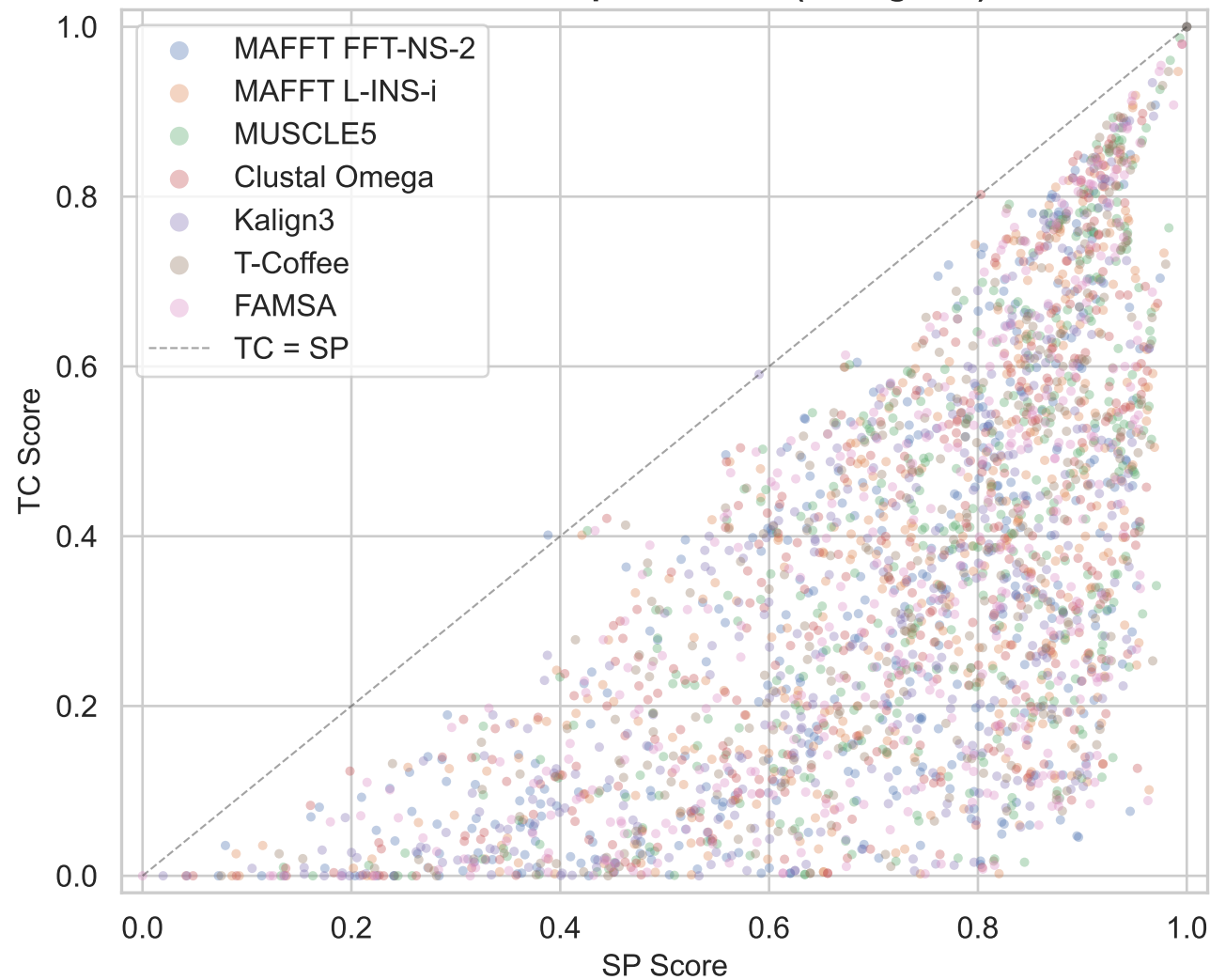
SP vs TC Score per Problem (all aligners)
