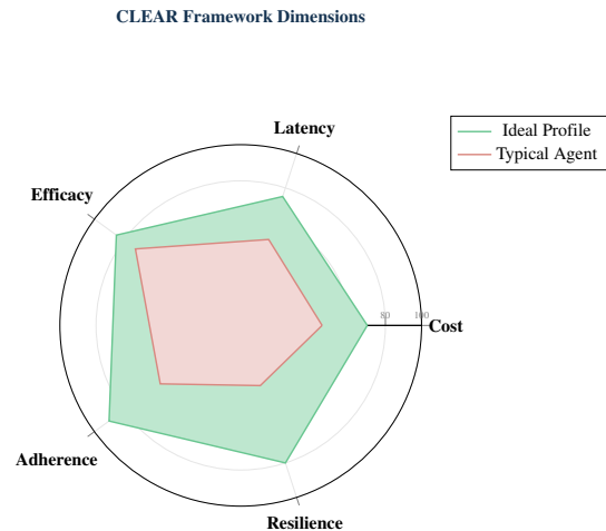
FIGURE 7. The CLEAR framework radar chart, comparing an ideal agent profile (high scores across all dimensions) against a typical production agent (with notable gaps in Adherence and Resilience).
