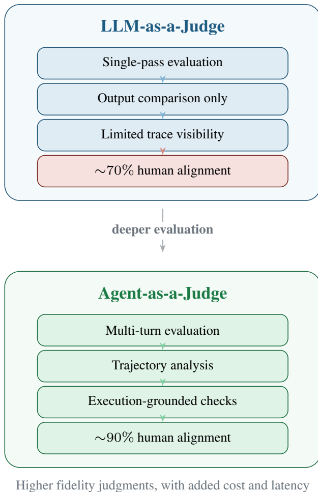
FIGURE 4. LLM-as-a-Judge vs. Agent-as-a-Judge comparison. Agent-as-a-Judge provides deeper process evaluation through multi-turn analysis and trajectory inspection, achieving significantly higher human alignment.
