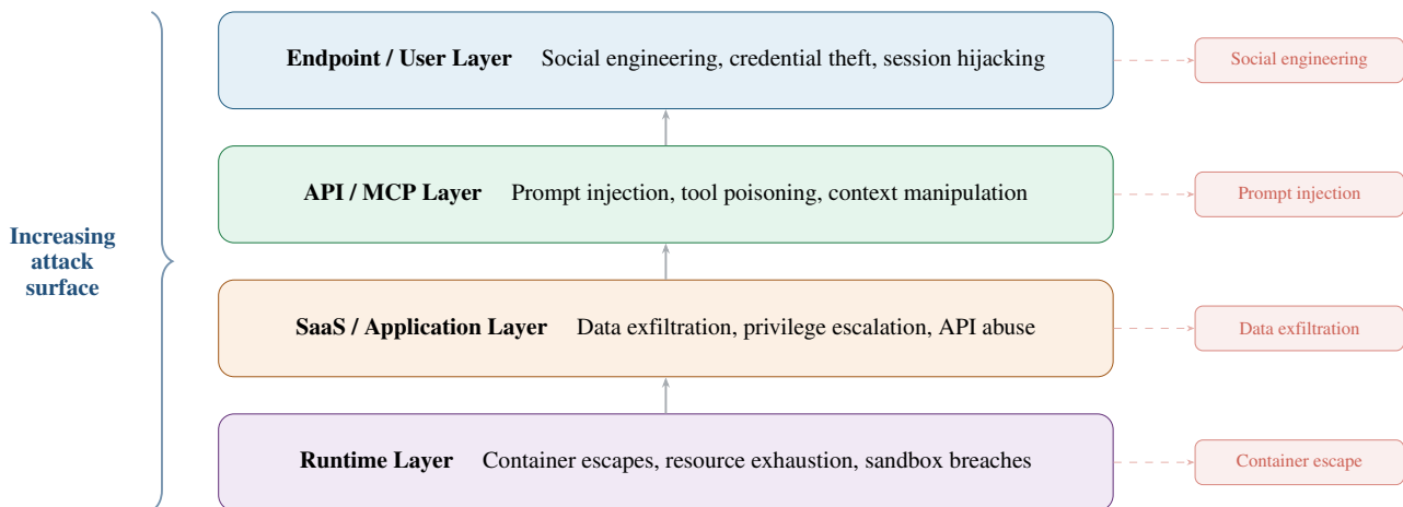
FIGURE 6. The four-layer security attack surface for agentic AI systems, from runtime infrastructure to endpoint users, with representative threat vectors at each layer.
