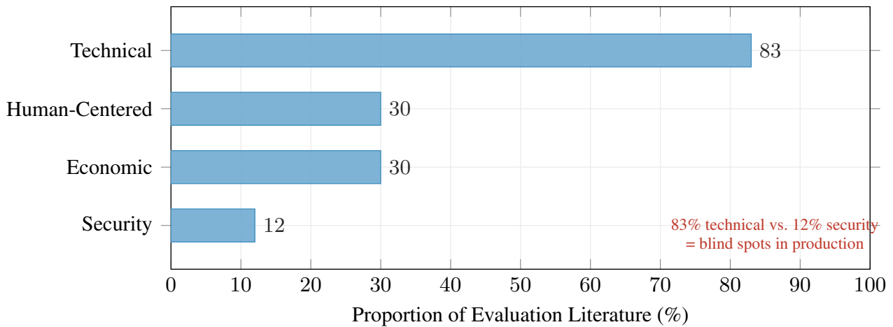
FIGURE 8. The measurement imbalance in agentic AI evaluation. Technical metrics dominate the literature, while security and human-centered considerations remain critically underrepresented.
