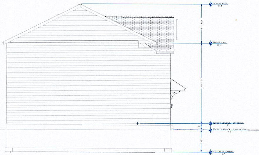
LEFT SIDE VIEW ELEVATION 1/4 IN = 1 FT
