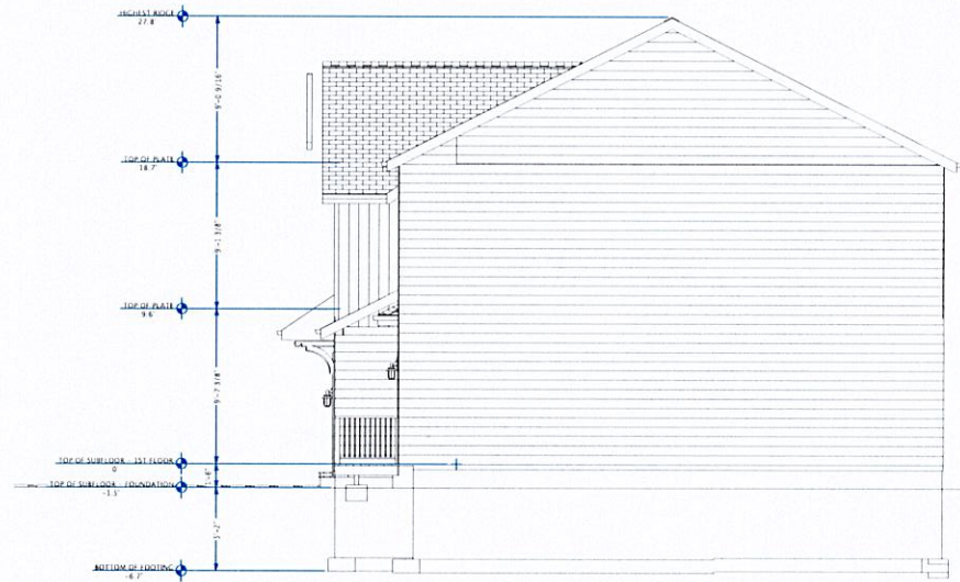
RIGHT SIDE VIEW ELEVATION 1/4 IN = 1 FT
