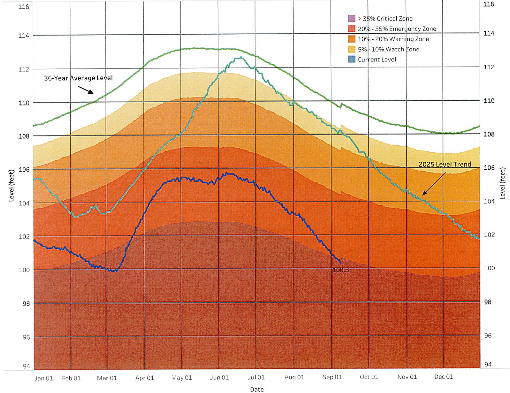
Kenoza Lake Drought Stages with Current, 2025, and Average Levels
