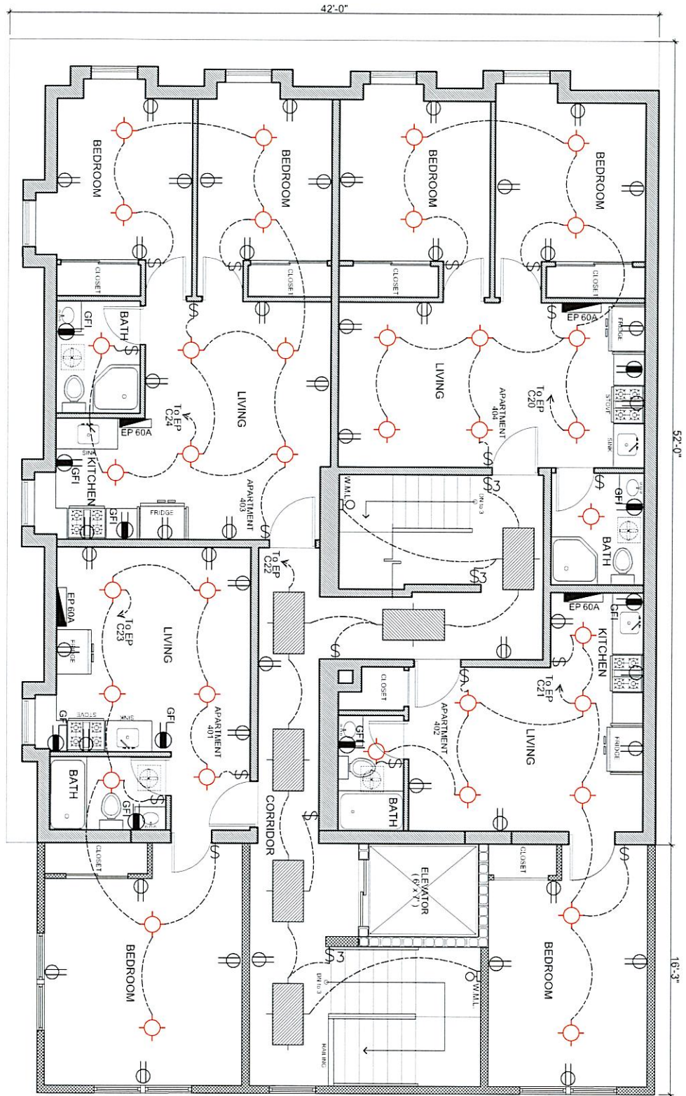
(ELECTRICAL) PROPOSED FOURTH FLOOR PLAN SCALE: 1/8"=1'-0"
