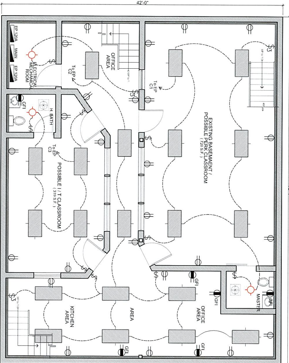
PROPOSED BASEMENT FLOOR PLAN (ELECTRICAL)
