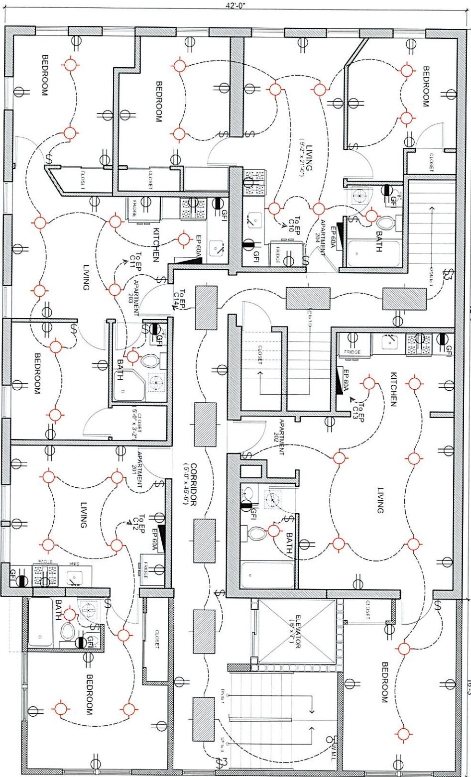
(ELECTRICAL) PROPOSED SECOND FLOOR PLAN
