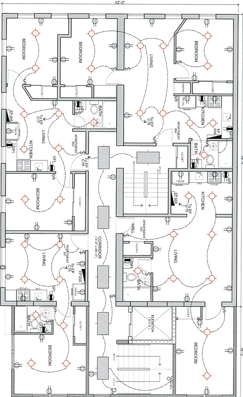
(ELECTRICAL) PROPOSED THIRD FLOOR PLAN
