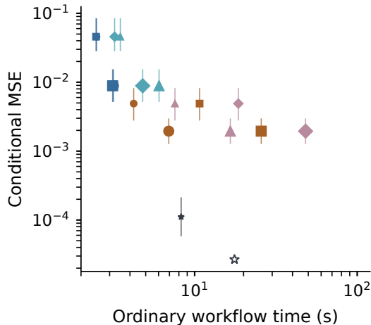
d H2: noncentred funnel, v / 3
