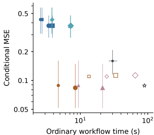
c H1: centred funnel, v / 3
