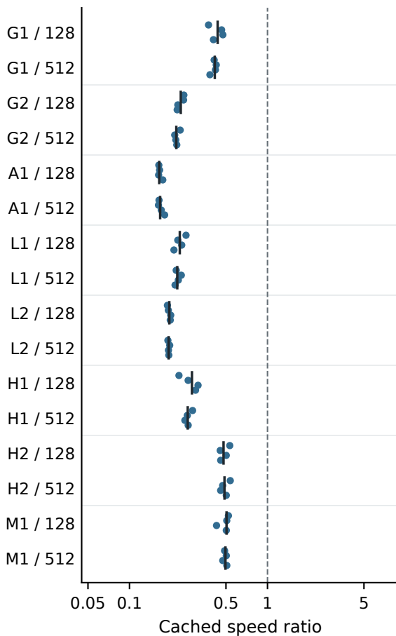
a quasi-DEER / MALA
