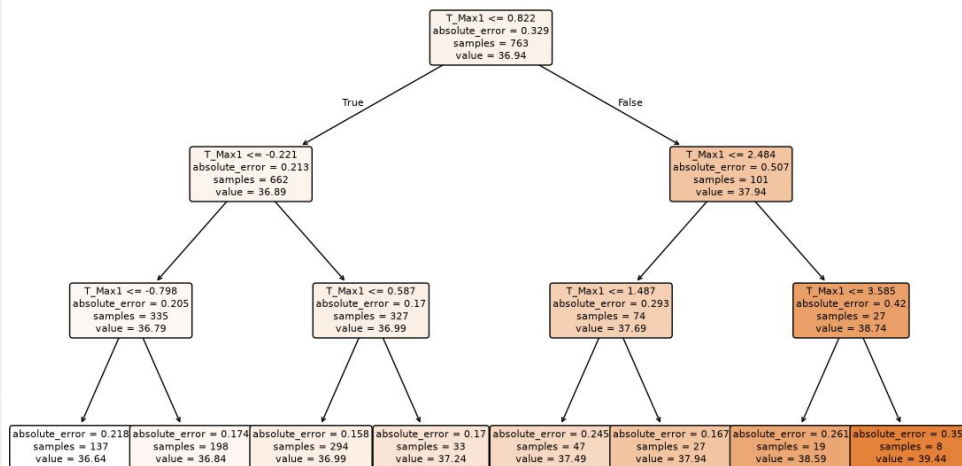
Decision Tree Regressor (best model)
