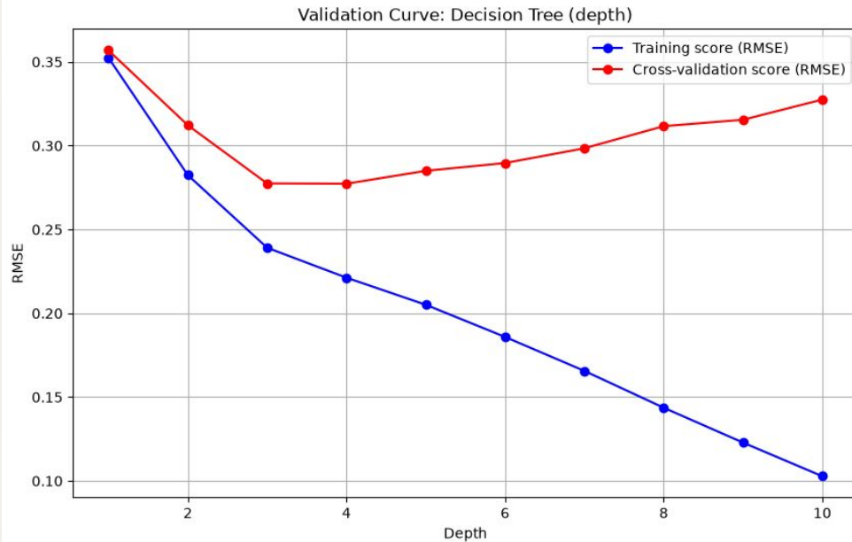
Decision Tree Regressor (best model)
