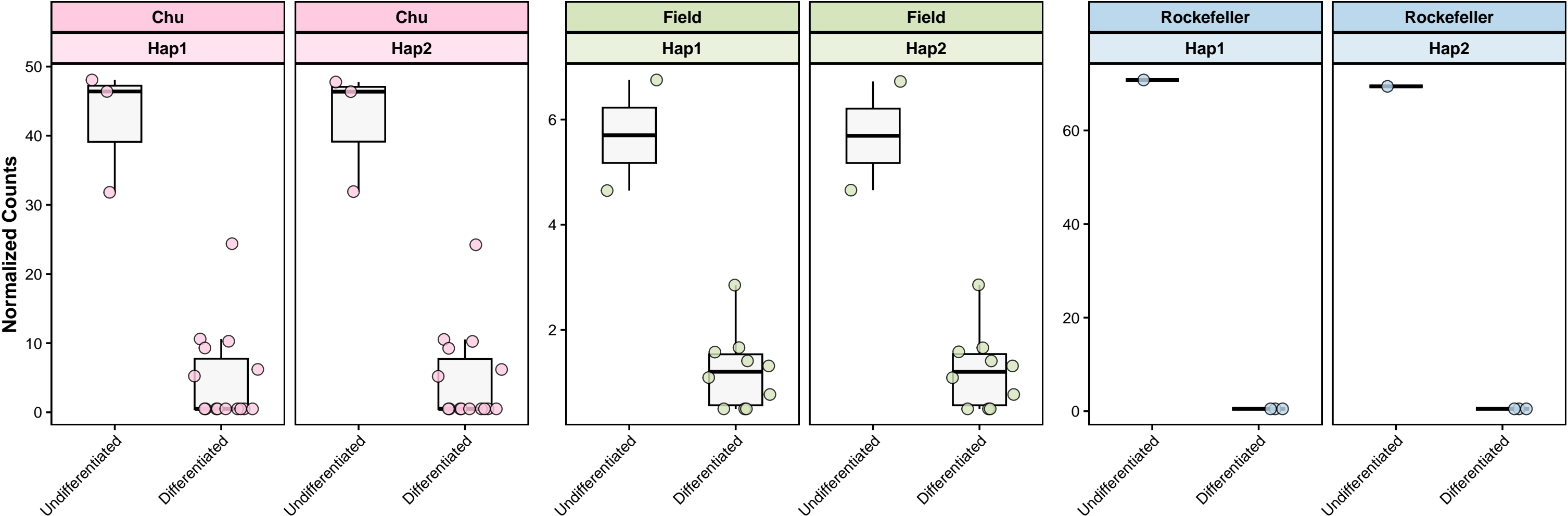
TERT Expression: TERT Comparison by Study and Haplotype
