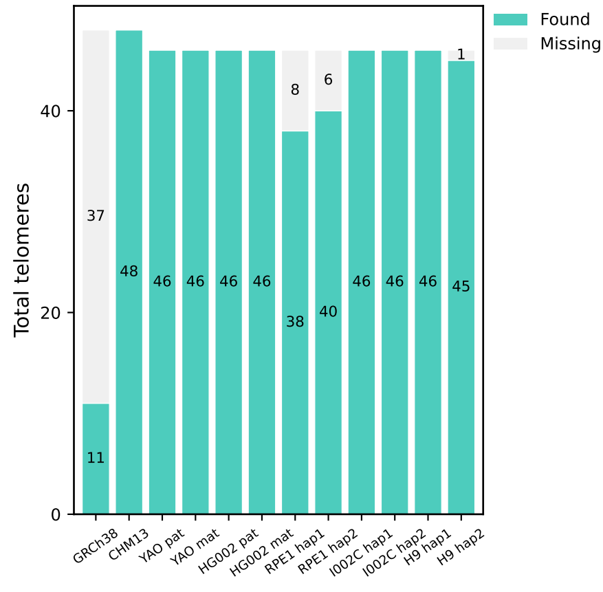
Assembly telomeres
