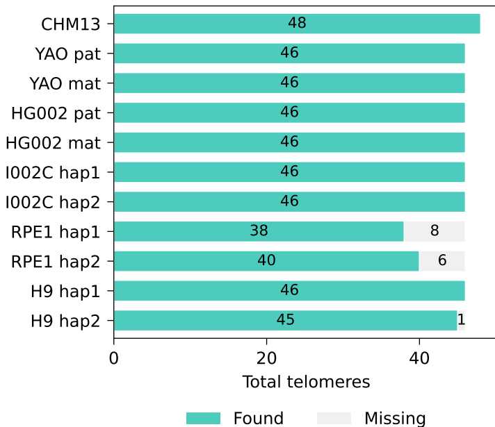
Assembly telomeres
