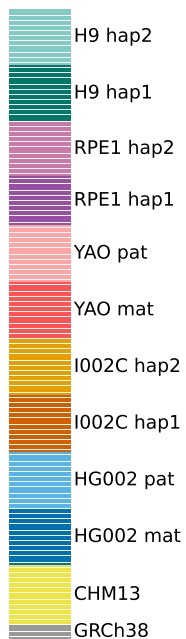
Canonical proportion (%)
