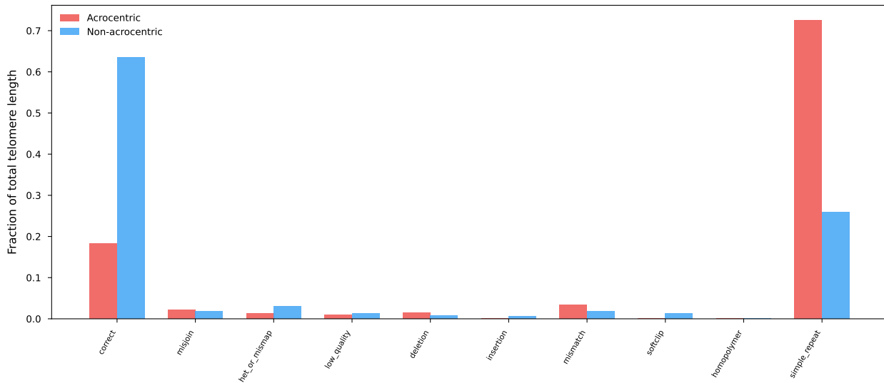
Acrocentric vs other (HiFi)
